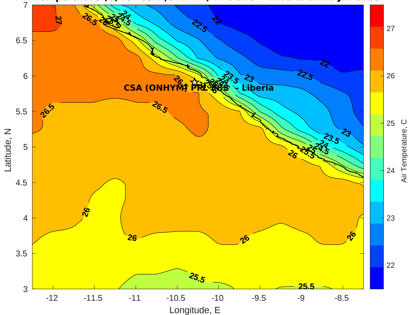
Air Temperature (C) for CSA (ONHYM) PPL EBS - Liberia at 10-Jul-2025
