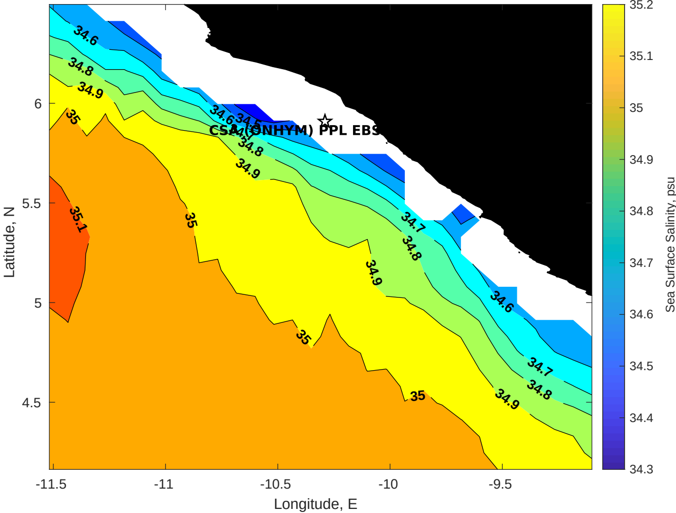
Surface Salinity for CSA (ONHYM) PPL EBS - Liberia at 09-Jul-2025 00:00:00
