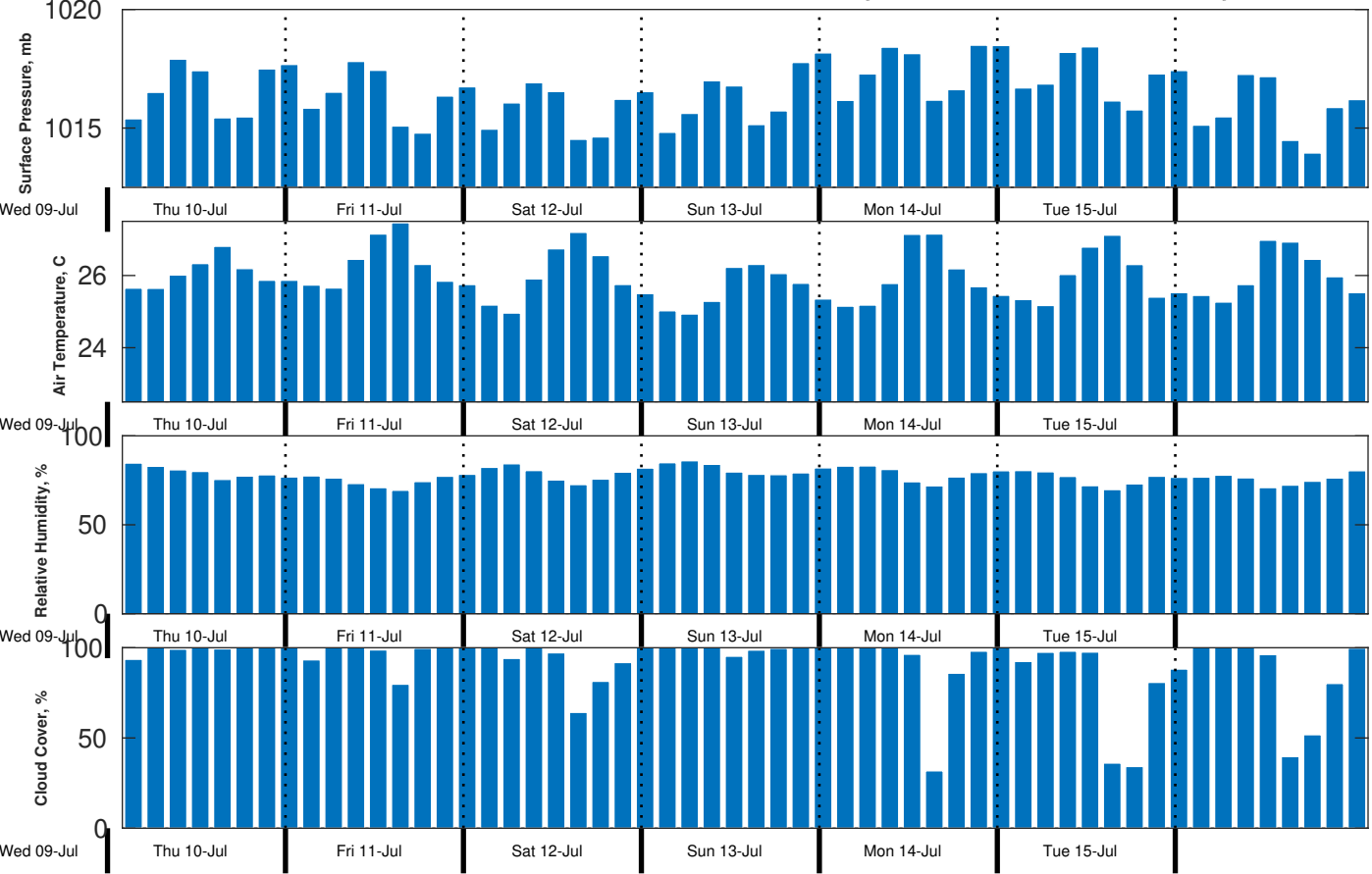
Met Forecast for CSA (ONHYM) PPL EBS - Liberia from 10-Jul-2025 00:00:00 to 17-Jul-2025 00:00:00
