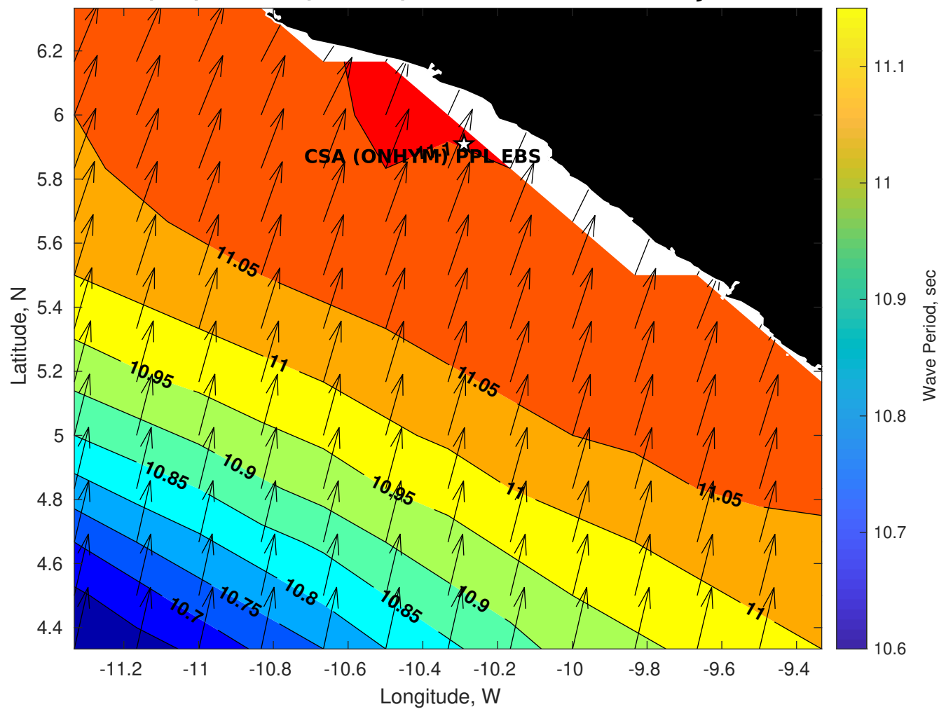
Wave Period (sec) for CSA (ONHYM) PPL EBS - Liberia at 10-Jul-2025 09:00:00
