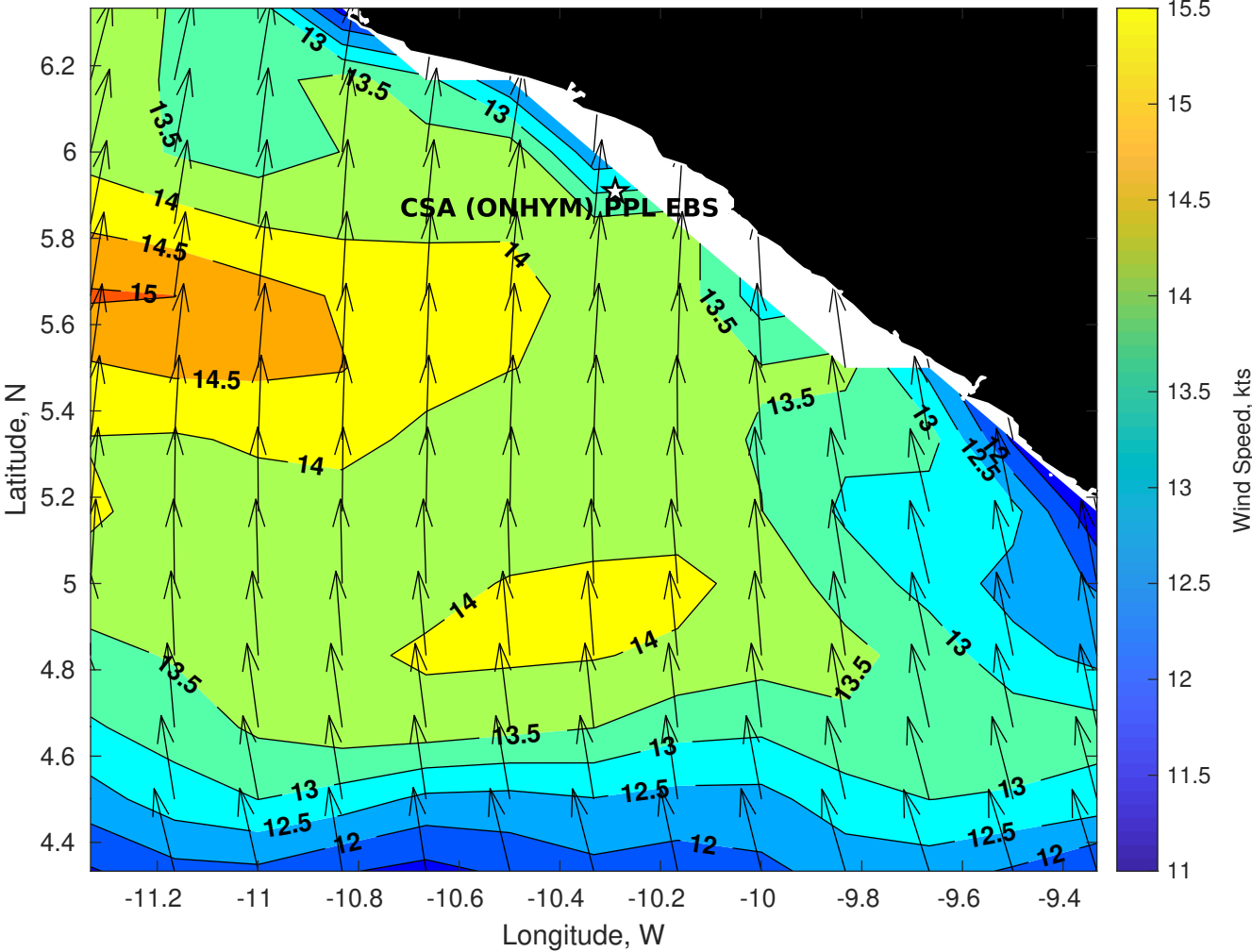
Winds (kts) for CSA (ONHYM) PPL EBS - Liberia at 10-Jul-2025 09:00:00
