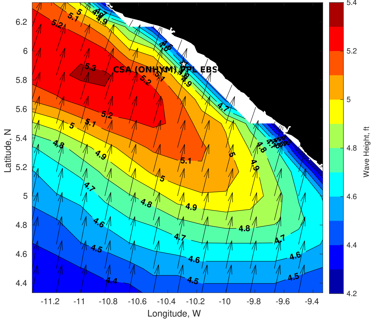
Wave Height (ft) for CSA (ONHYM) PPL EBS - Liberia at 10-Jul-2025 09:00:00
