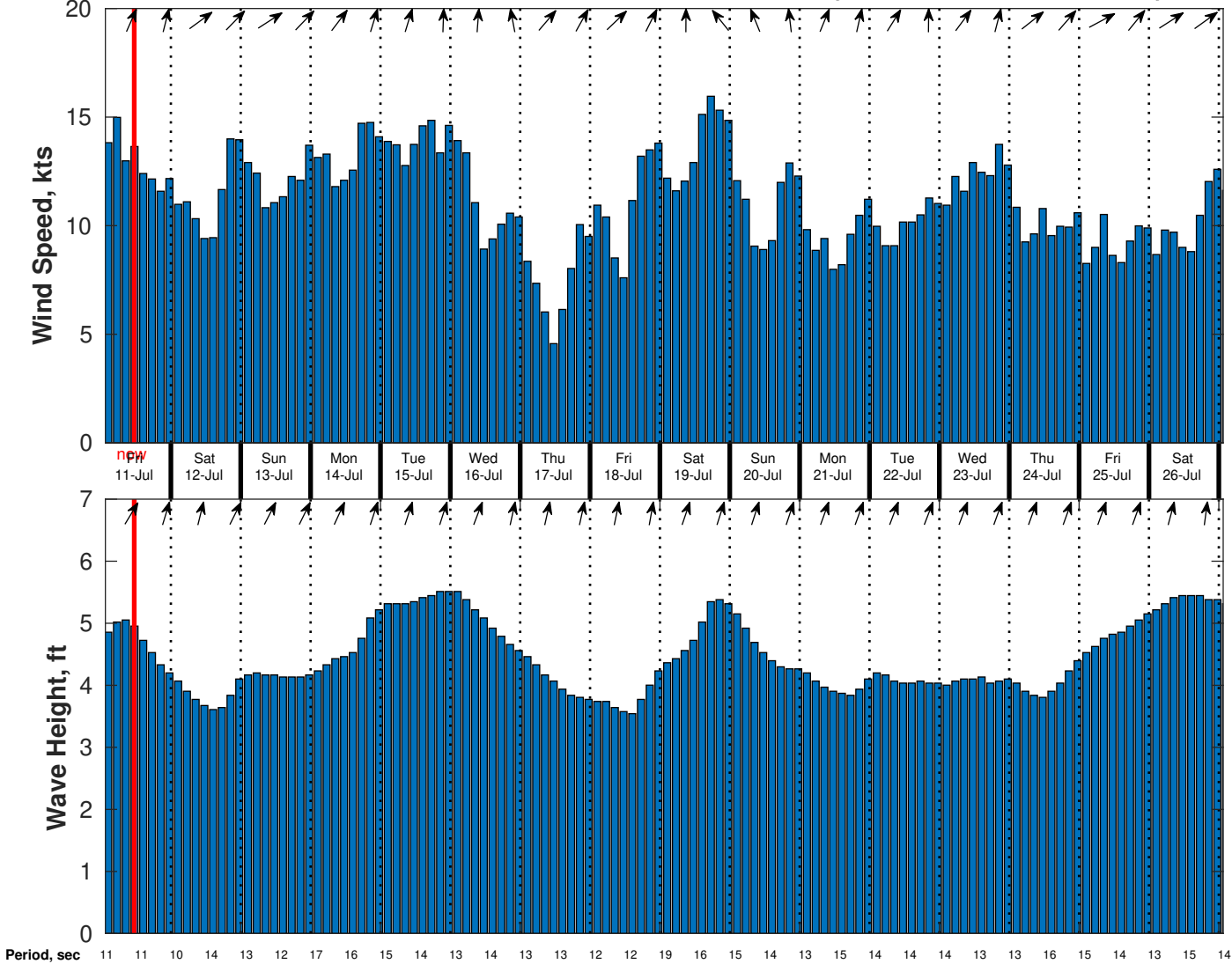
Wind & Wave Forecast for CSA (ONHYM) PPL EBS - Liberia from 10-Jul-2025 01:00:00 to 26-Jul-2025 01:00:00
