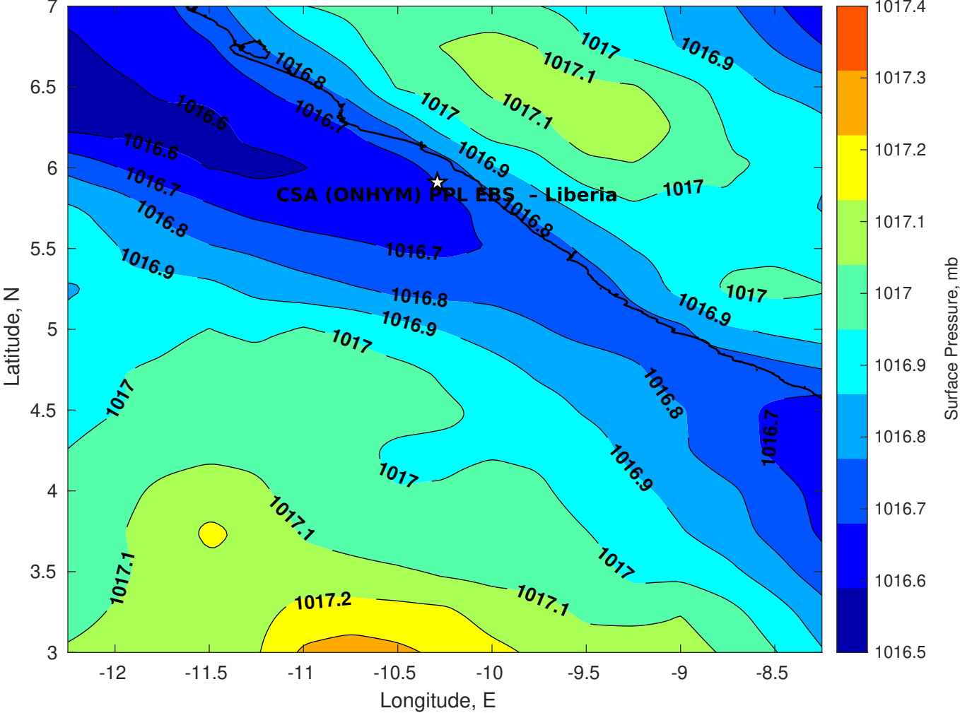
Surface Pressure (mb) for CSA (ONHYM) PPL EBS - Liberia at 12-Jul-2025 00:00:00
