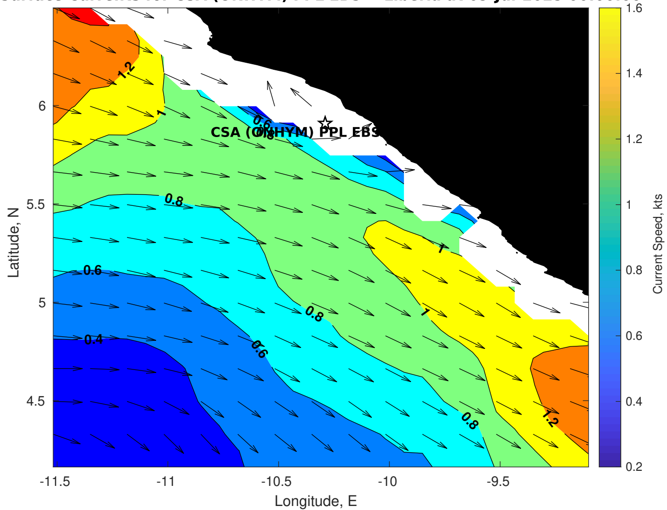
Surface Currents for CSA (ONHYM) PPL EBS - Liberia at 09-Jul-2025 00:00:00
