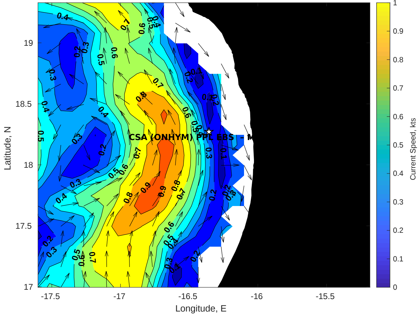
Surface Currents for CSA (ONHYM) PPL EBS - Mauritania at 09-Jul-2025 00:00:00
