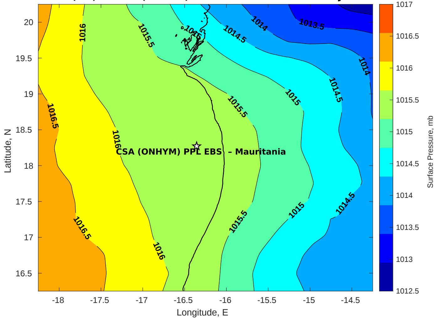
Surface Pressure (mb) for CSA (ONHYM) PPL EBS - Mauritania at 10-Jul-2025 00:00:00
