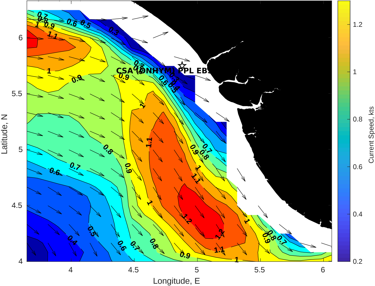
Surface Currents for CSA (ONHYM) PPL EBS - Nigeria at 09-Jul-2025 00:00:00
