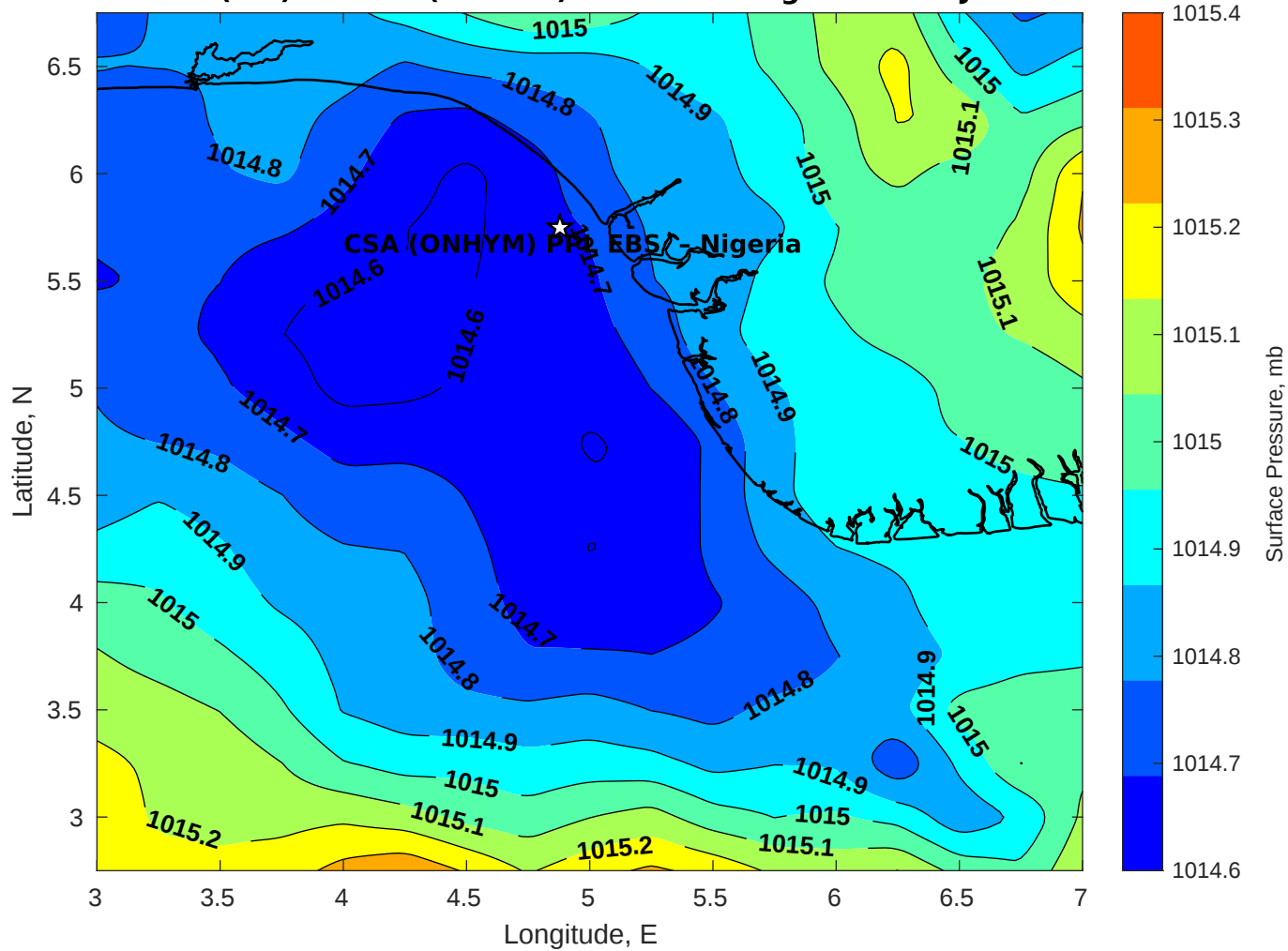
Surface Pressure (mb) for CSA (ONHYM) PPL EBS - Nigeria at 12-Jul-2025 00:00:00
