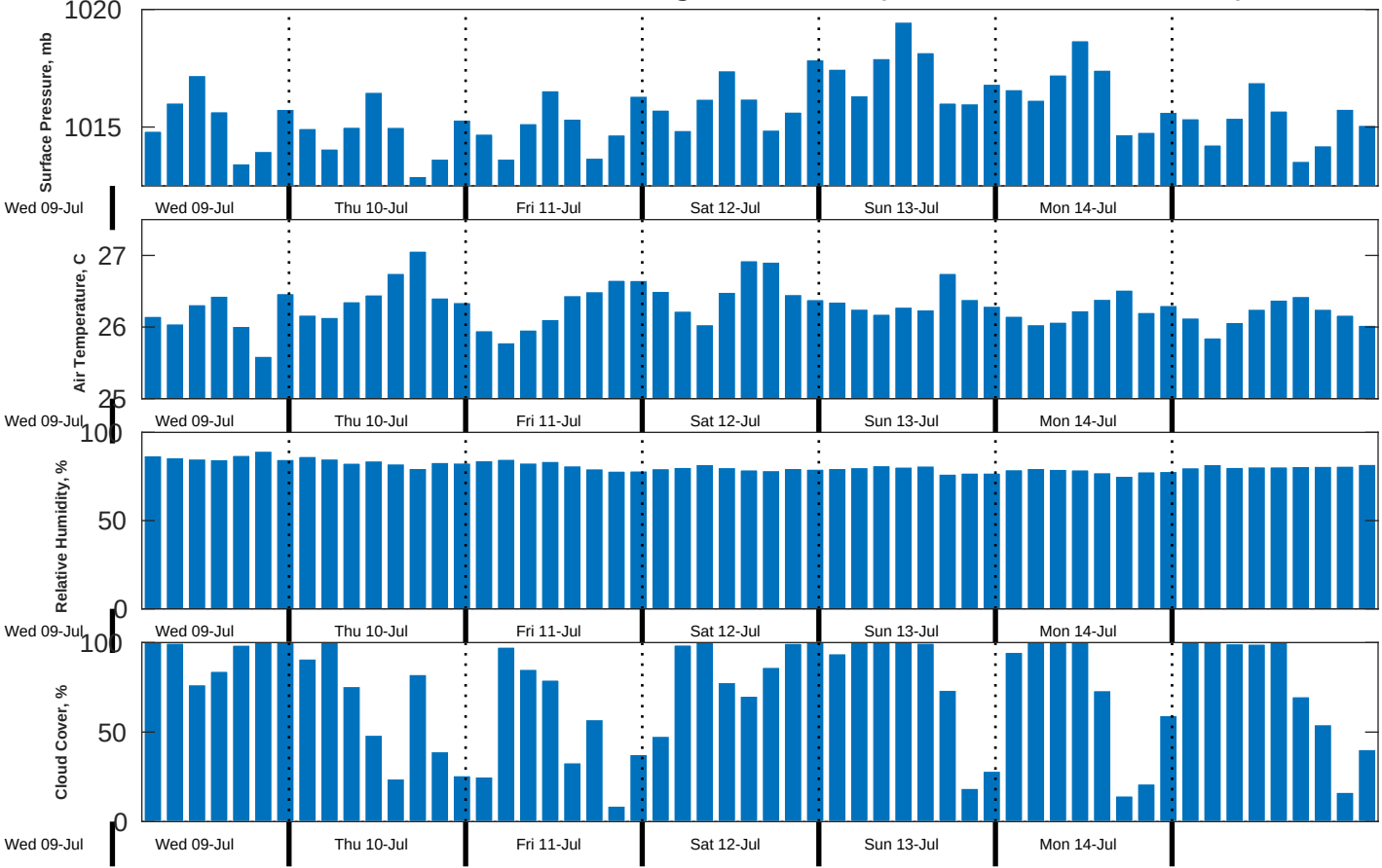
Met Forecast for CSA (ONHYM) PPL EBS - Nigeria from 10-Jul-2025 00:00:00 to 17-Jul-2025 00:00:00
