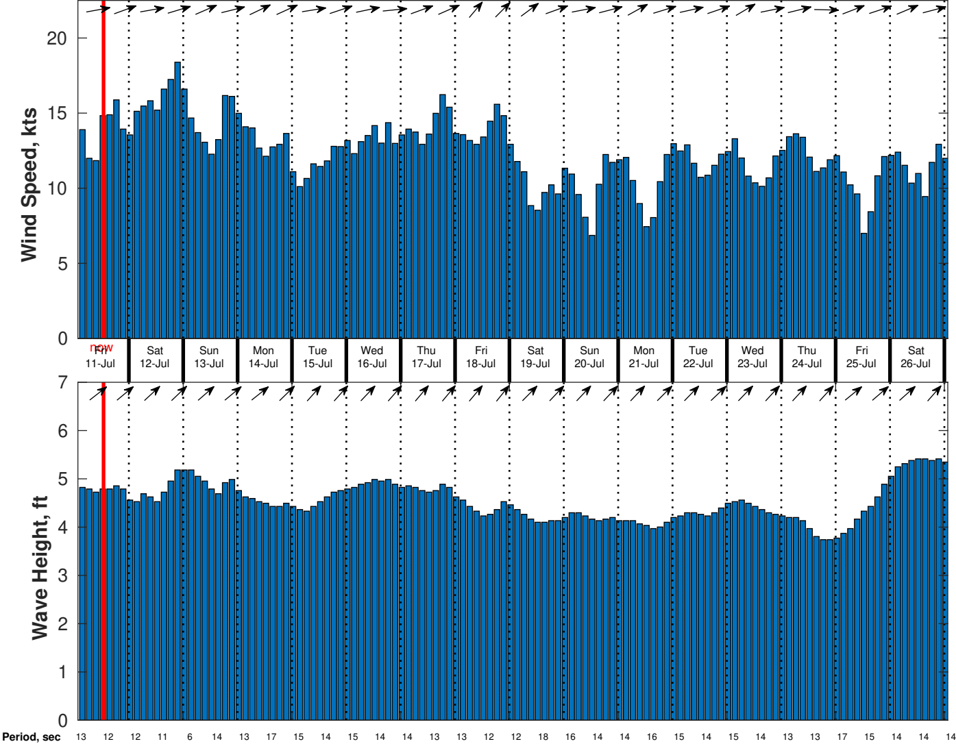
Wind & Wave Forecast for CSA (ONHYM) PPL EBS - Nigeria from 10-Jul-2025 02:00:00 to 26-Jul-2025 02:00:00
