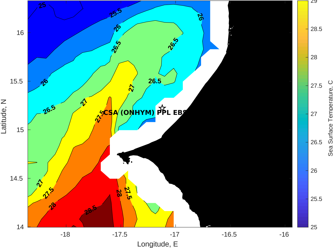
SST for CSA (ONHYM) PPL EBS - Senegal at 09-Jul-2025 00:00:00
