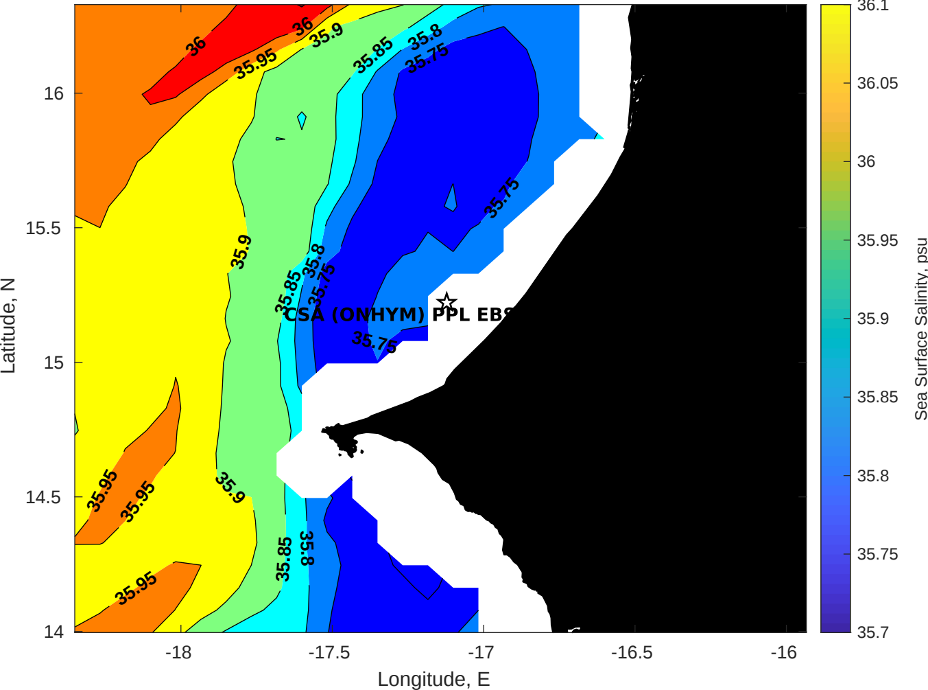
Surface Salinity for CSA (ONHYM) PPL EBS - Senegal at 09-Jul-2025 00:00:00
