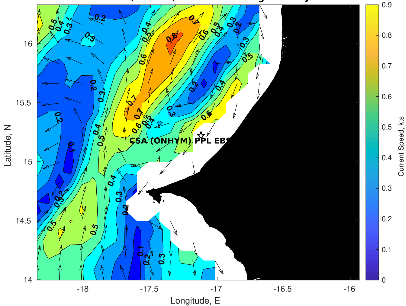
Surface Currents for CSA (ONHYM) PPL EBS - Senegal at 09-Jul-2025 00:00:00
