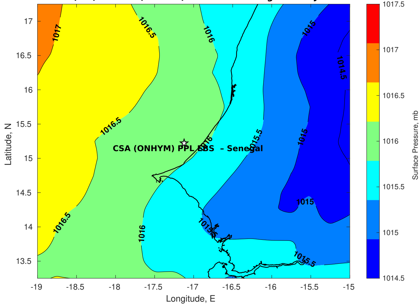
Surface Pressure (mb) for CSA (ONHYM) PPL EBS - Senegal at 10-Jul-2025 00:00:00
