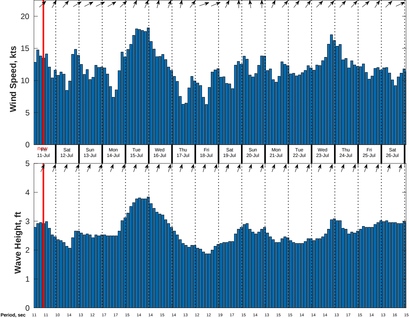
Wind & Wave Forecast for CSA (ONHYM) PPL EBS - Sierra Leone from 10-Jul-2025 01:00:00 to 26-Jul-2025 01:00:00
