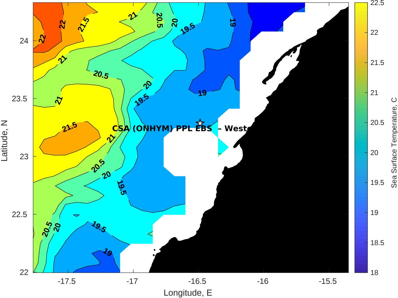
SST for CSA (ONHYM) PPL EBS - Western Sahara at 09-Jul-2025 00:00:00
