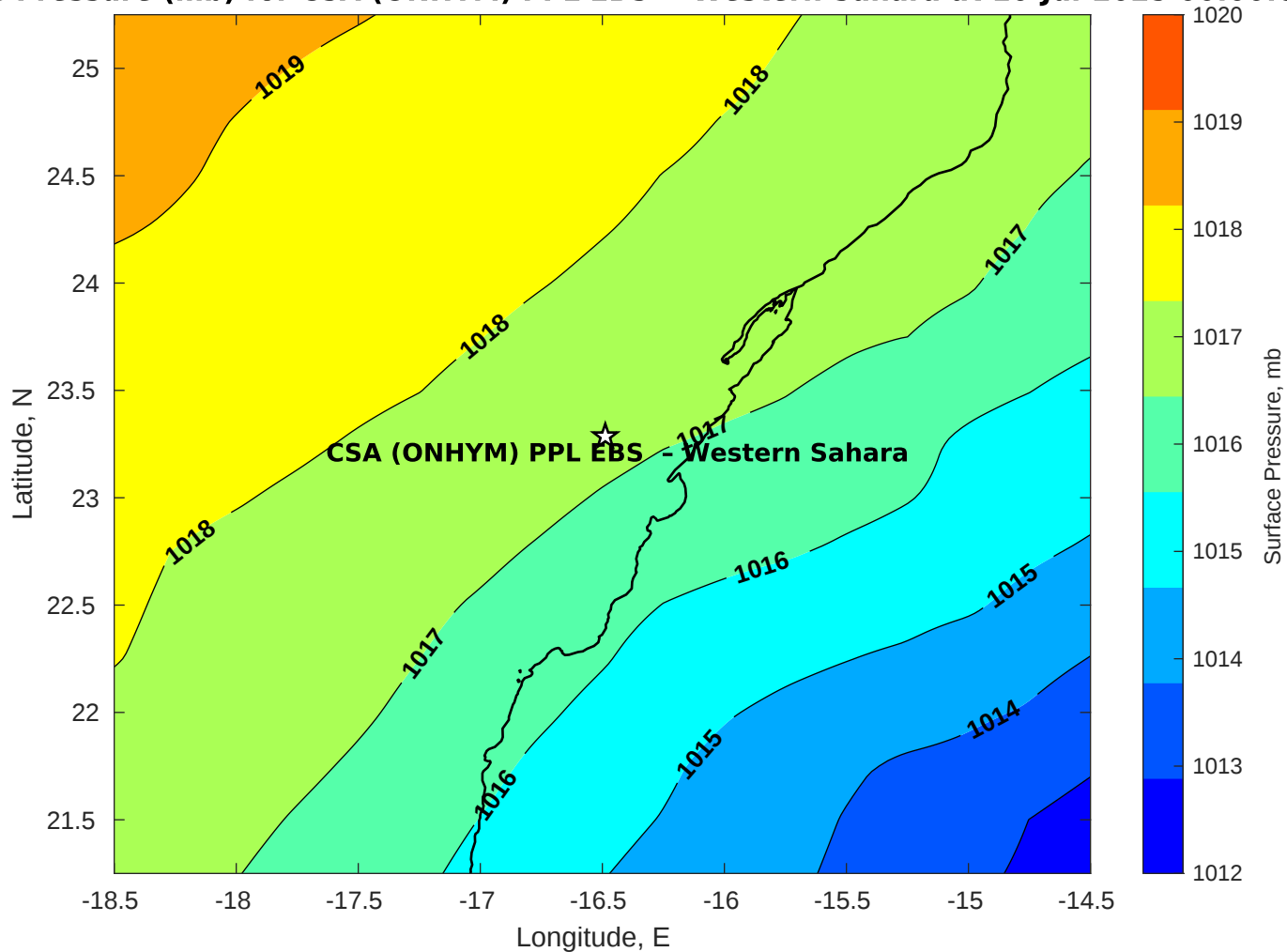
Surface Pressure (mb) for CSA (ONHYM) PPL EBS - Western Sahara at 10-Jul-2025 00:00:00
