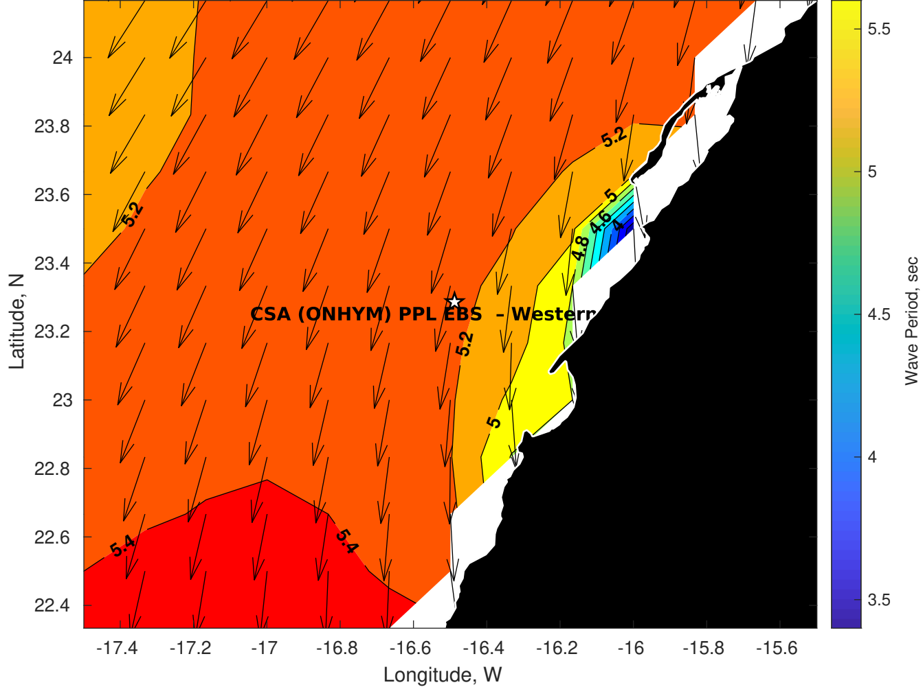
Wave Period (sec) for CSA (ONHYM) PPL EBS - Western Sahara at 10-Jul-2025 09:00:00
