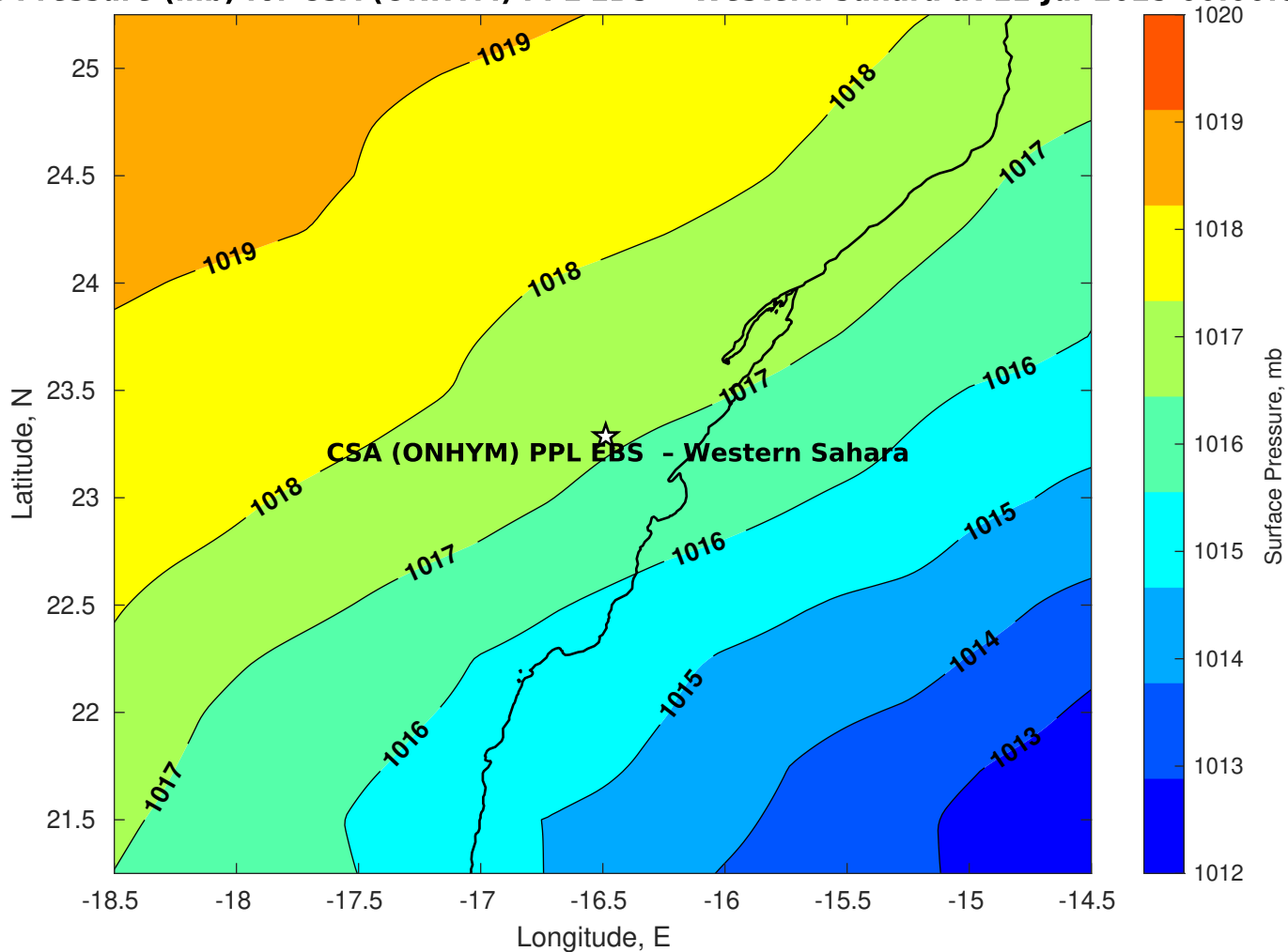
Surface Pressure (mb) for CSA (ONHYM) PPL EBS - Western Sahara at 11-Jul-2025 00:00:00
