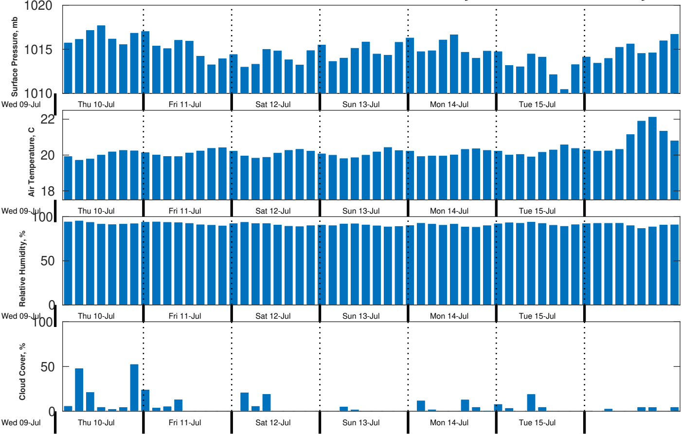
Met Forecast for CSA (ONHYM) PPL EBS - Western Sahara from 10-Jul-2025 00:00:00 to 17-Jul-2025 00:00:00
