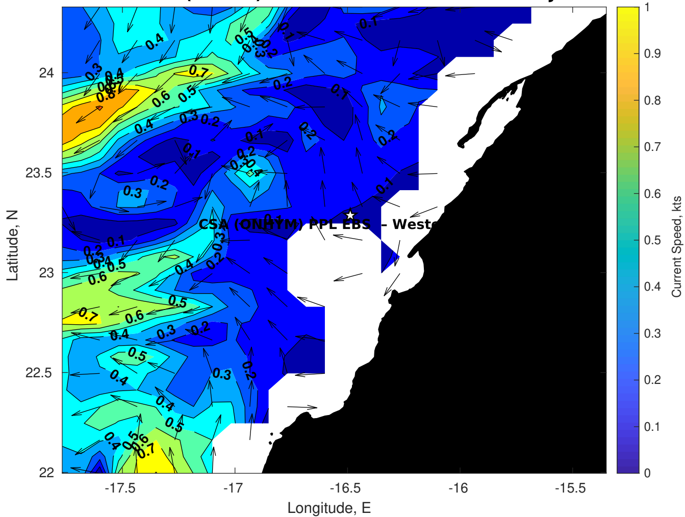
Surface Currents for CSA (ONHYM) PPL EBS - Western Sahara at 09-Jul-2025 00:00:00
