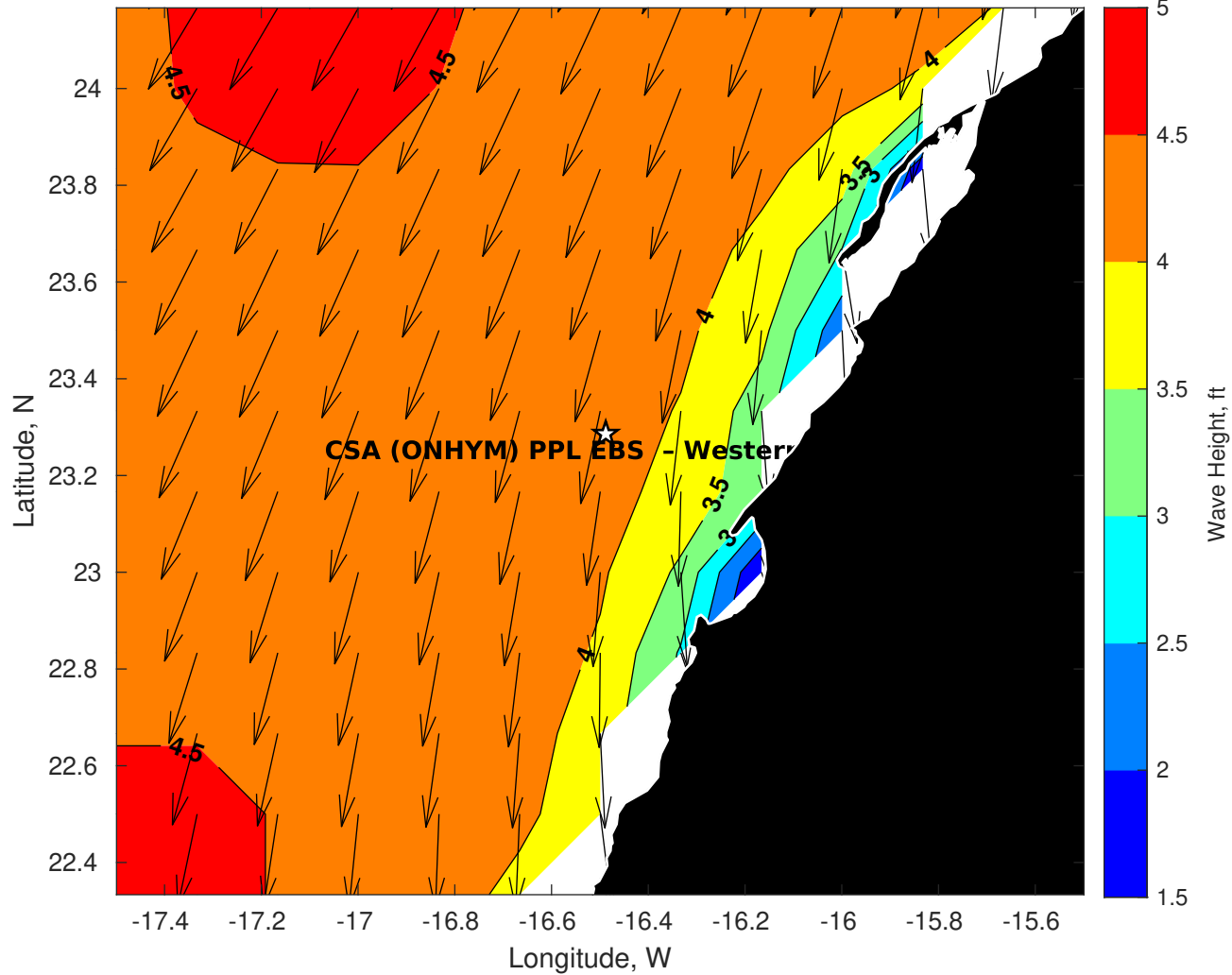
Wave Height (ft) for CSA (ONHYM) PPL EBS - Western Sahara at 10-Jul-2025 09:00:00
