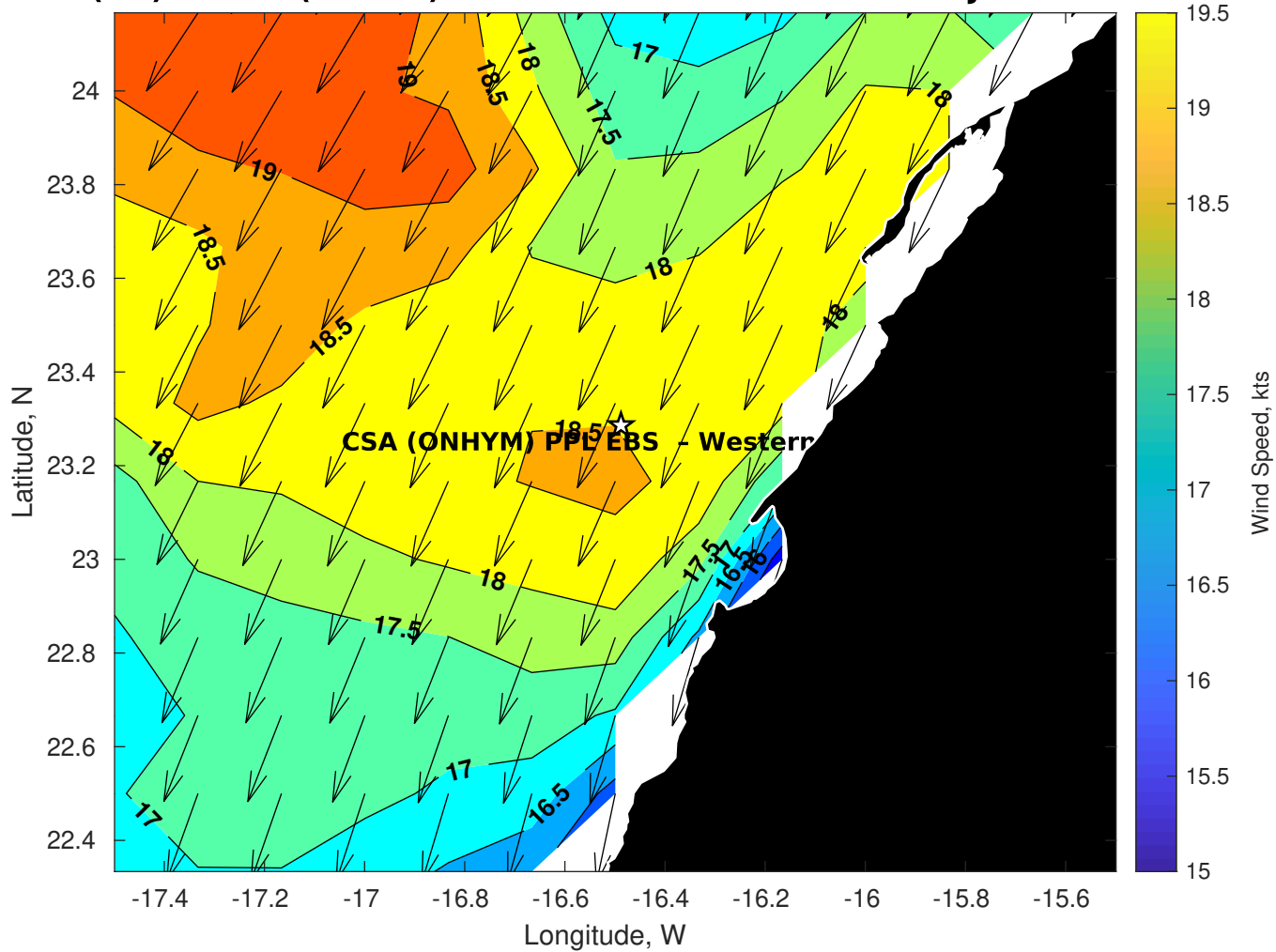
Winds (kts) for CSA (ONHYM) PPL EBS - Western Sahara at 10-Jul-2025 09:00:00
