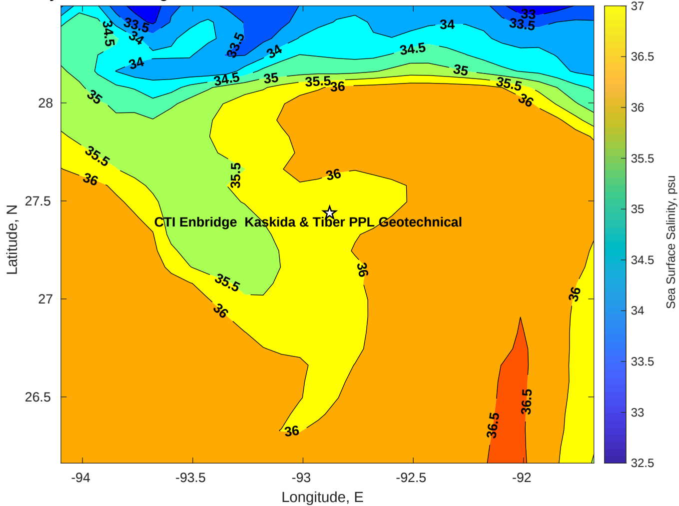
Surface Salinity for CTI Enbridge Kaskida & Tiber PPL Geotechnical at 09-Jul-2025 00:00:00
