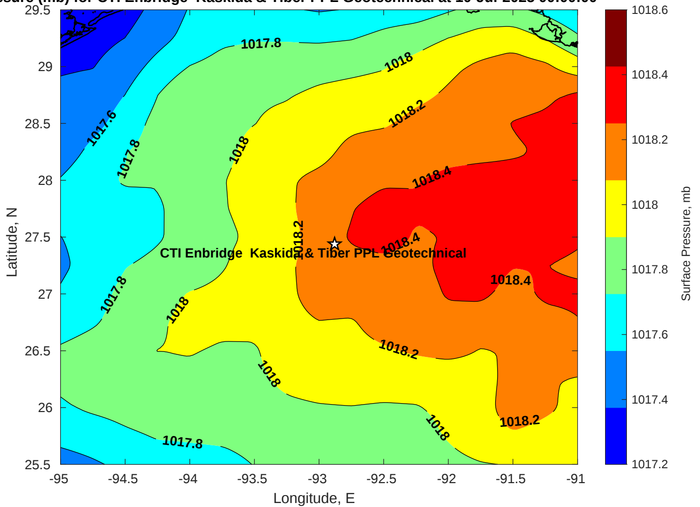
Surface Pressure (mb) for CTI Enbridge Kaskida & Tiber PPL Geotechnical at 10-Jul-2025 00:00:00
