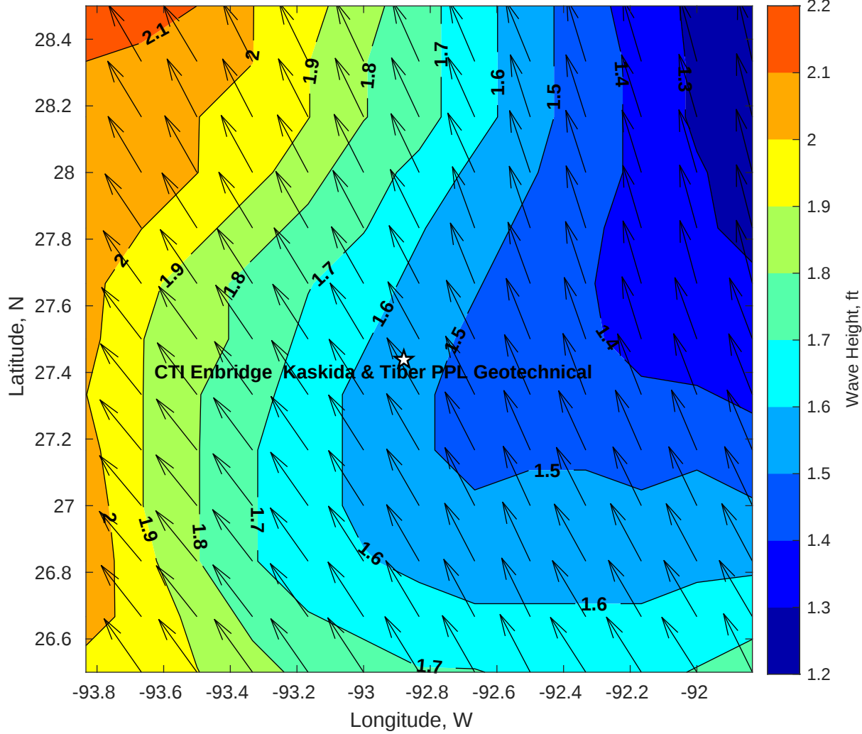
Wave Height (ft) for CTI Enbridge Kaskida & Tiber PPL Geotechnical at 10-Jul-2025 09:00:00
