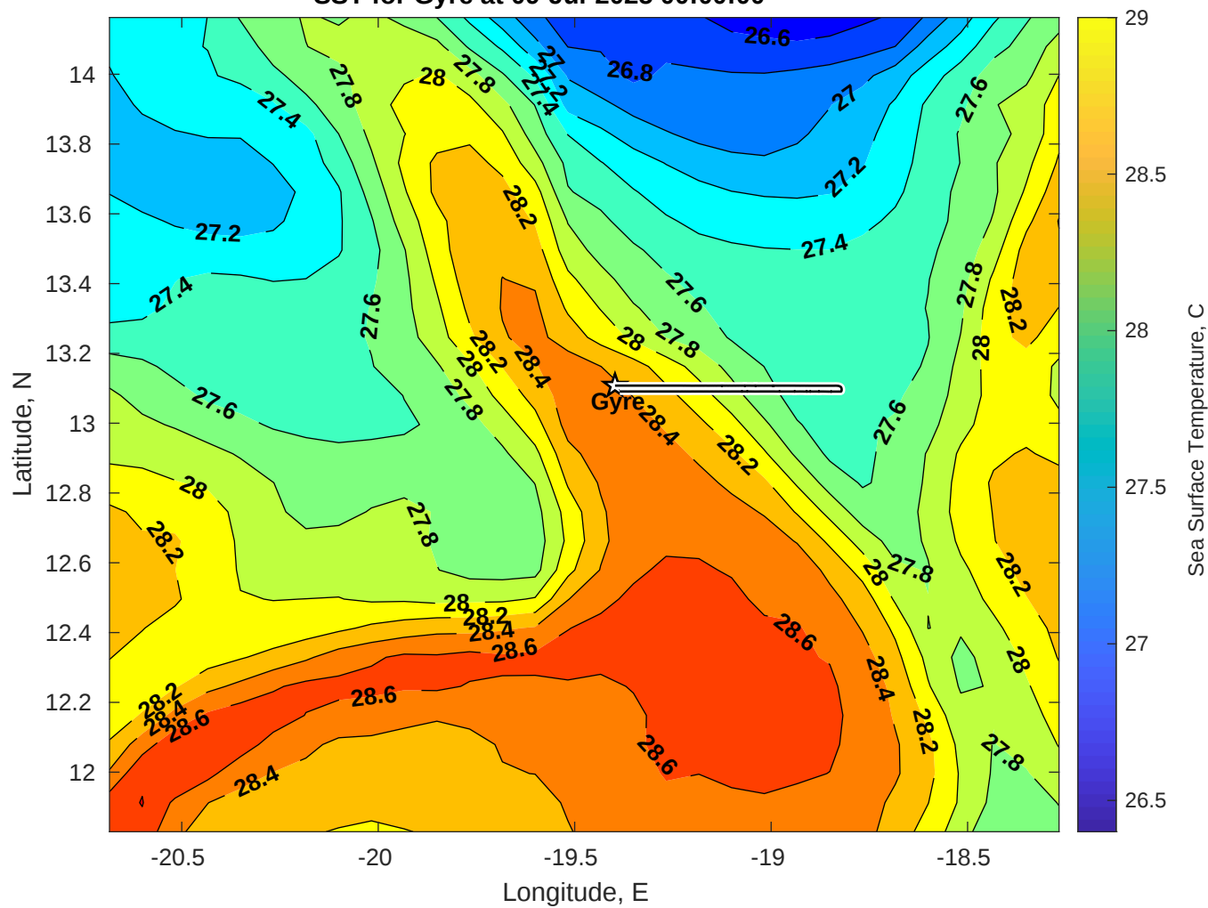
SST for Gyre at 09-Jul-2025 00:00:00
