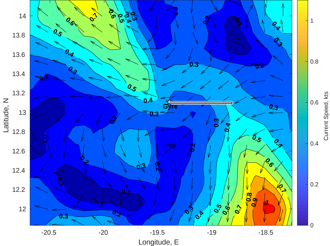
Surface Currents for Gyre at 09-Jul-2025 00:00:00
