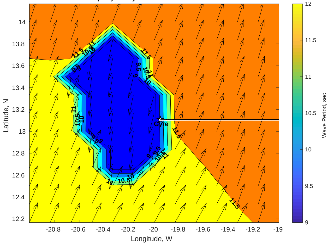
Wave Period (sec) for Gyre at 10-Jul-2025 09:00:00
