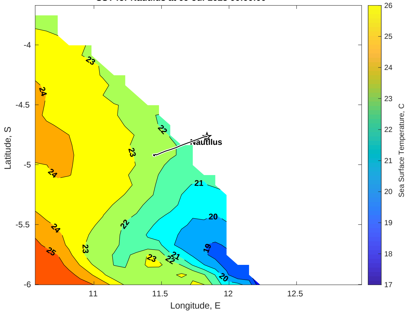
SST for Nautilus at 09-Jul-2025 00:00:00
