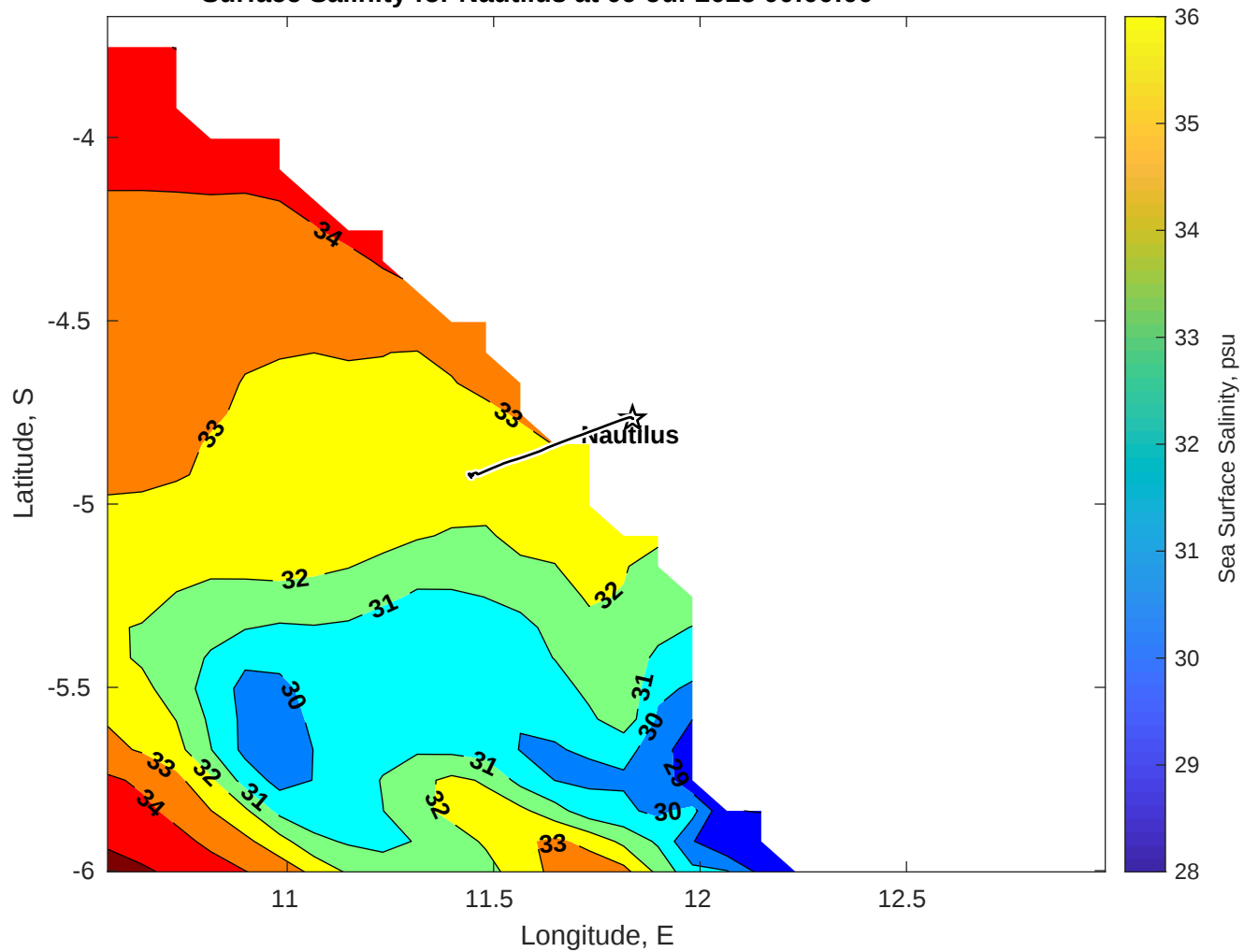
Surface Salinity for Nautilus at 09-Jul-2025 00:00:00
