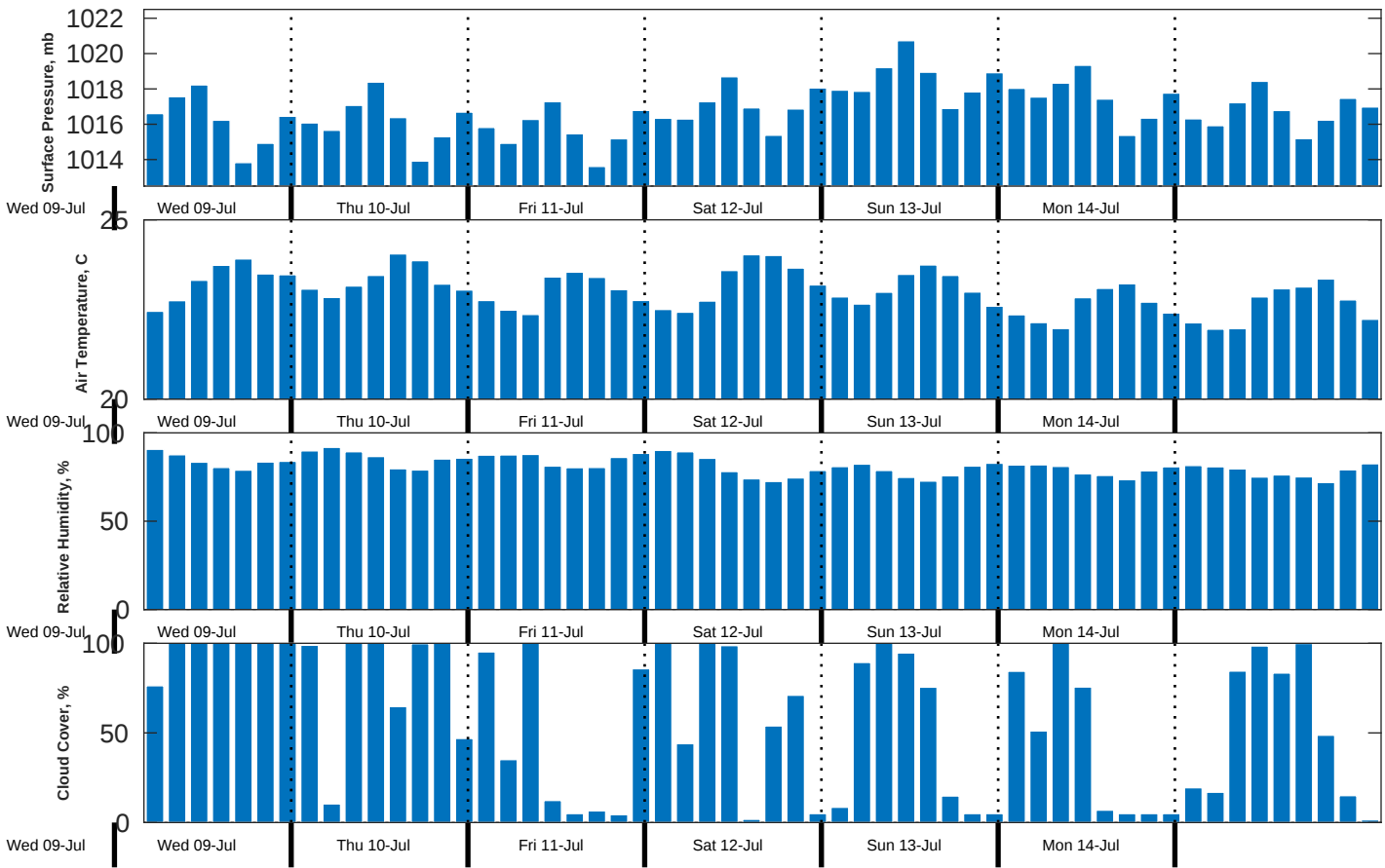
Met Forecast for Nautilus from 10-Jul-2025 00:00:00 to 17-Jul-2025 00:00:00
