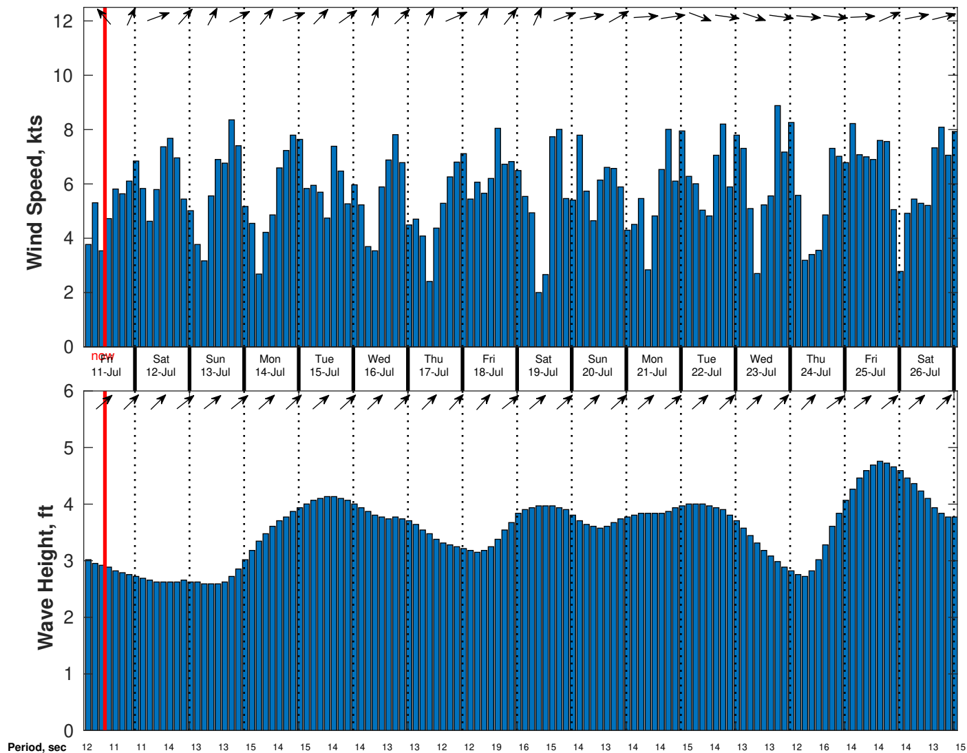
Wind & Wave Forecast for Nautilus from 10-Jul-2025 02:00:00 to 26-Jul-2025 02:00:00
