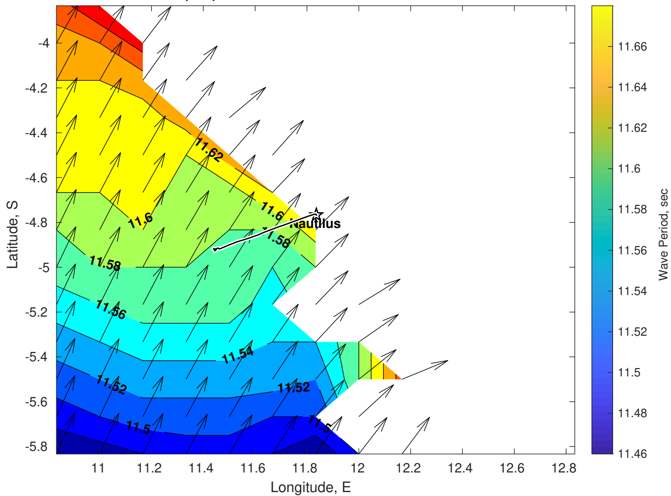
Wave Period (sec) for Nautilus at 10-Jul-2025 09:00:00
