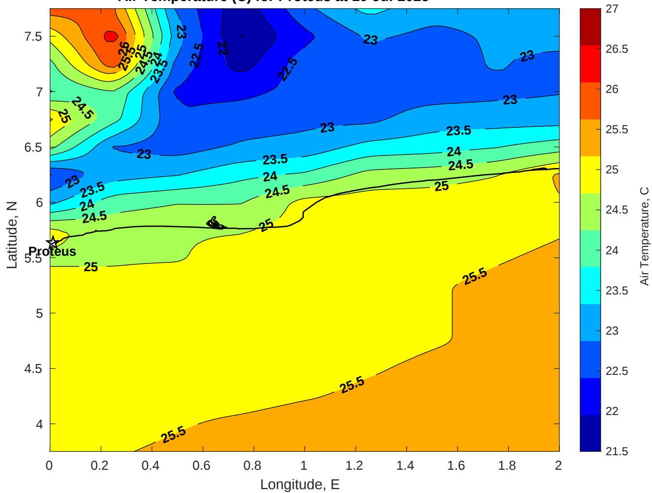
Air Temperature (C) for Proteus at 10-Jul-2025
