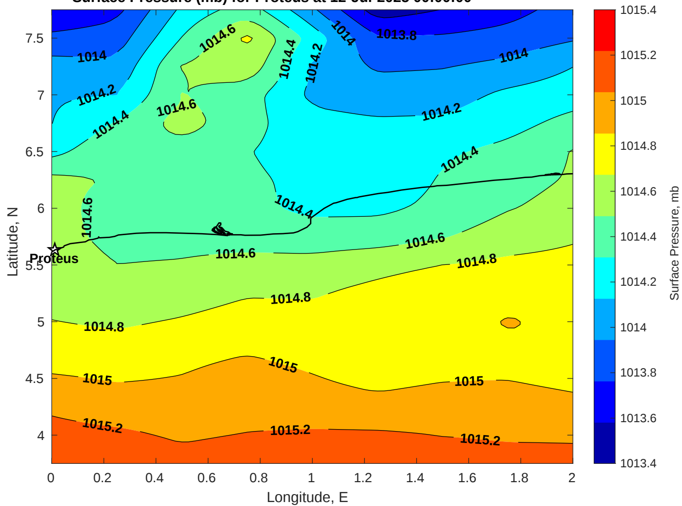
Surface Pressure (mb) for Proteus at 12-Jul-2025 00:00:00
