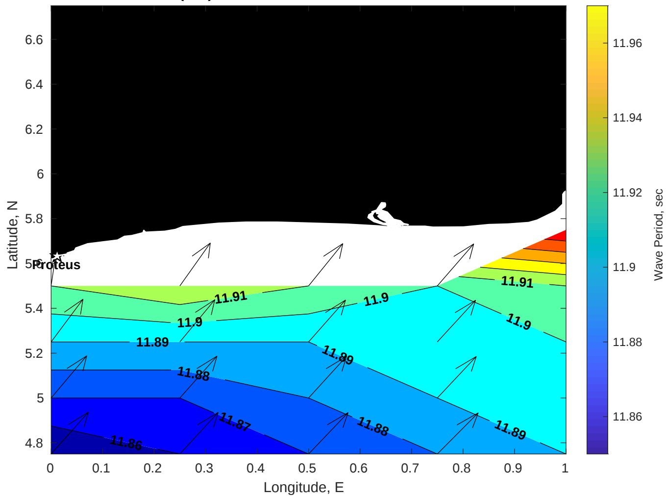
Wave Period (sec) for Proteus at 10-Jul-2025 09:00:00
