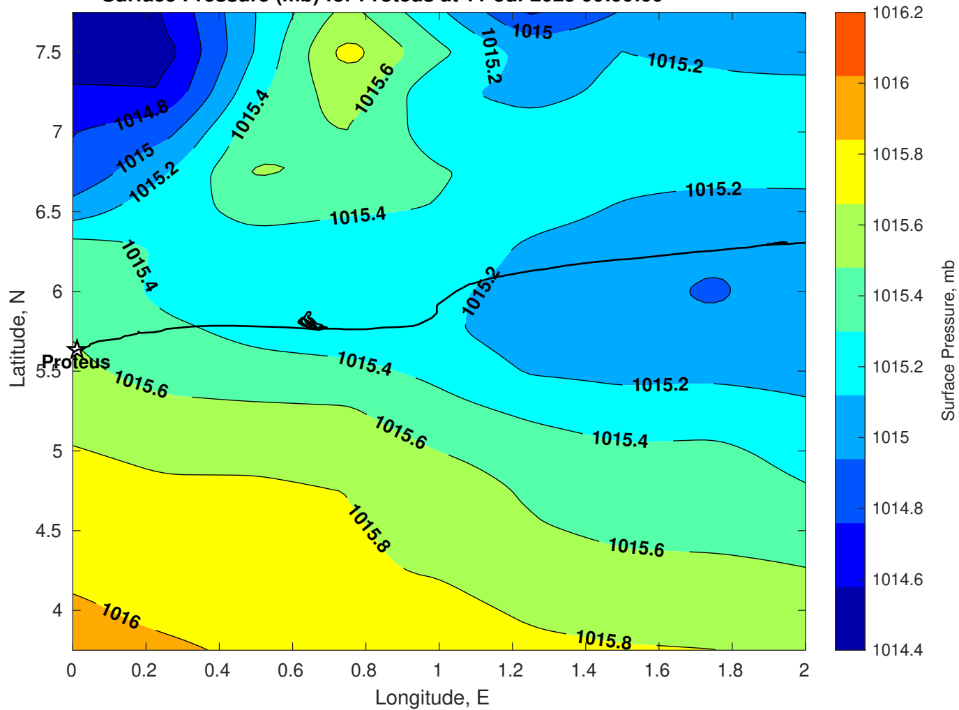
Surface Pressure (mb) for Proteus at 11-Jul-2025 00:00:00
