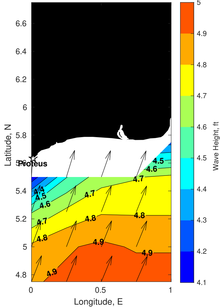
Wave Height (ft) for Proteus at 10-Jul-2025 09:00:00
