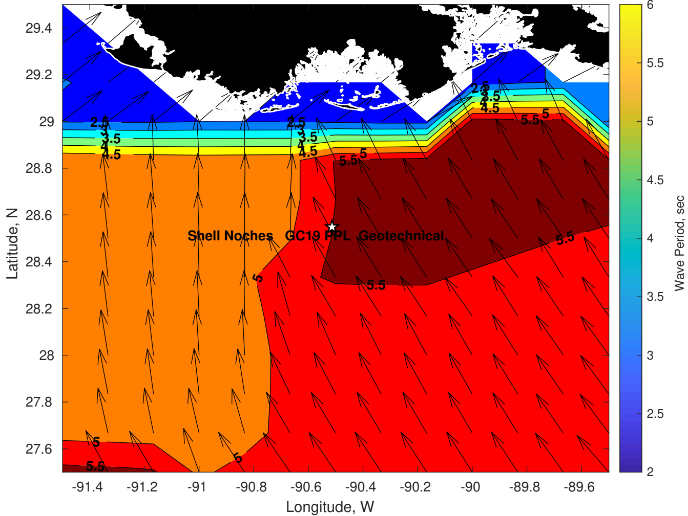
Wave Period (sec) for Shell Noches GC19 PPL Geotechnical at 10-Jul-2025 09:00:00
