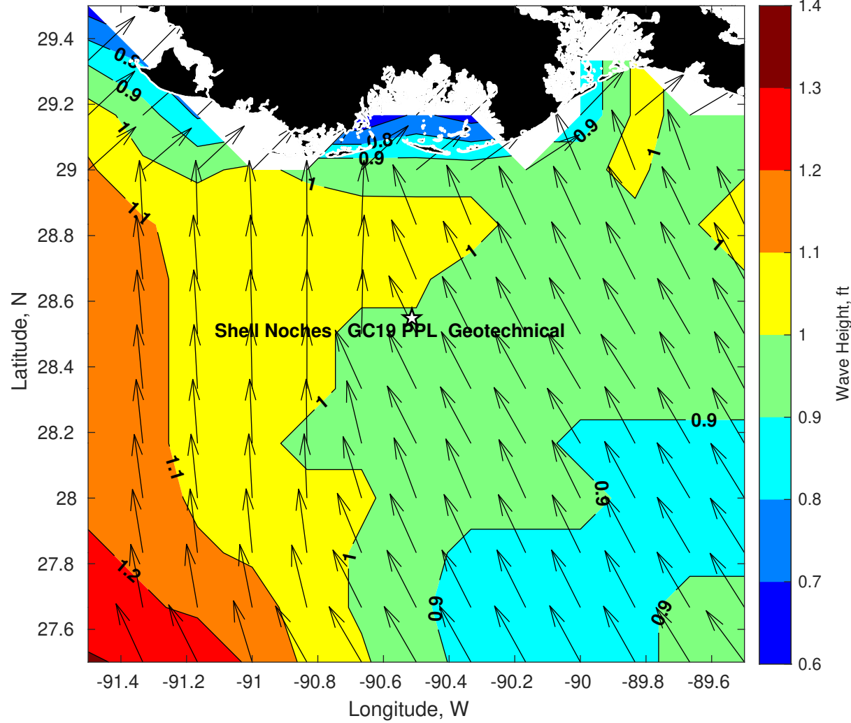
Wave Height (ft) for Shell Noches GC19 PPL Geotechnical at 10-Jul-2025 09:00:00
