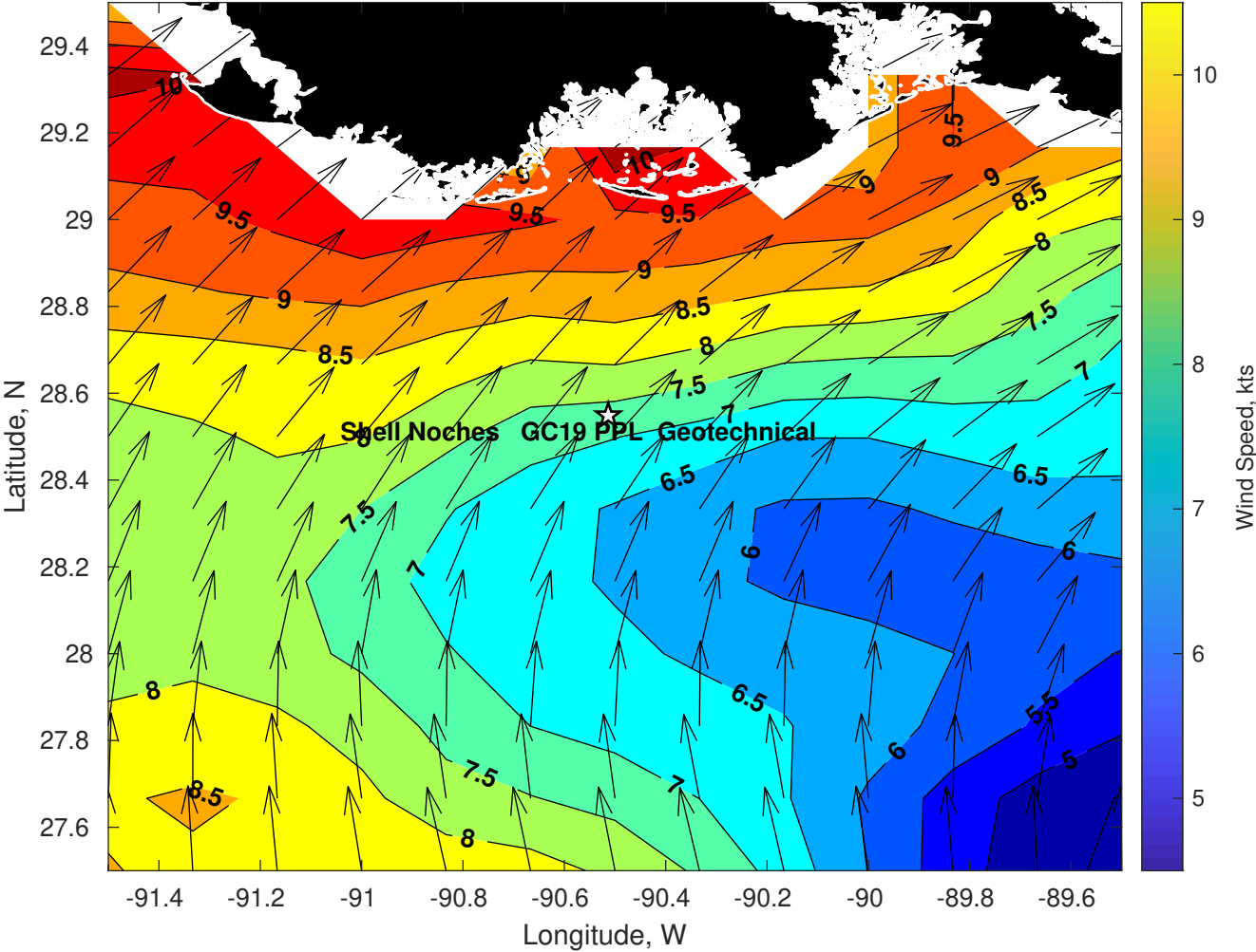
Winds (kts) for Shell Noches GC19 PPL Geotechnical at 10-Jul-2025 09:00:00
