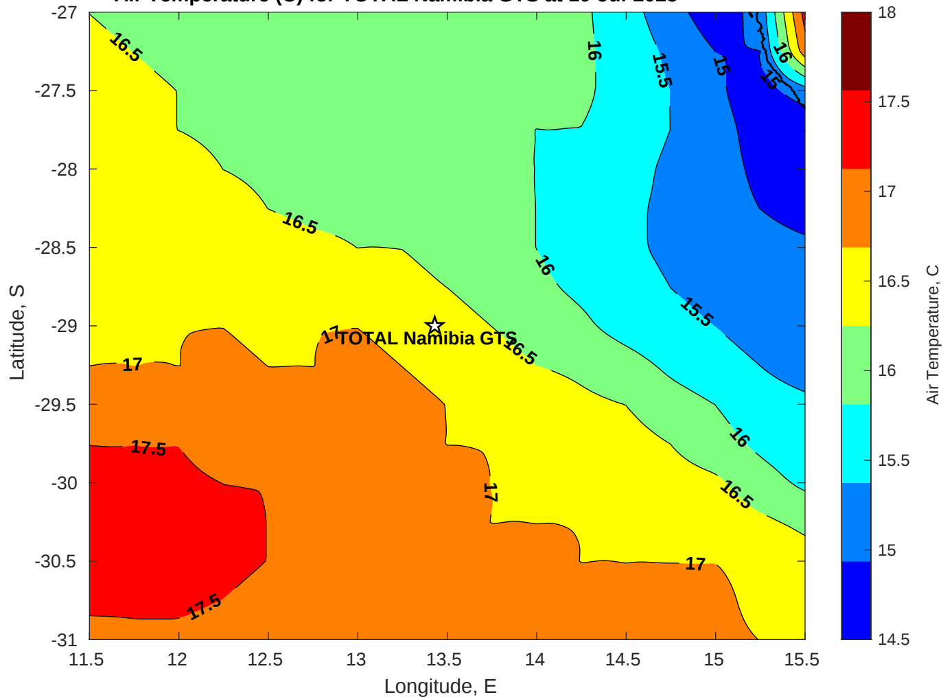
Air Temperature (C) for TOTAL Namibia GTS at 10-Jul-2025
