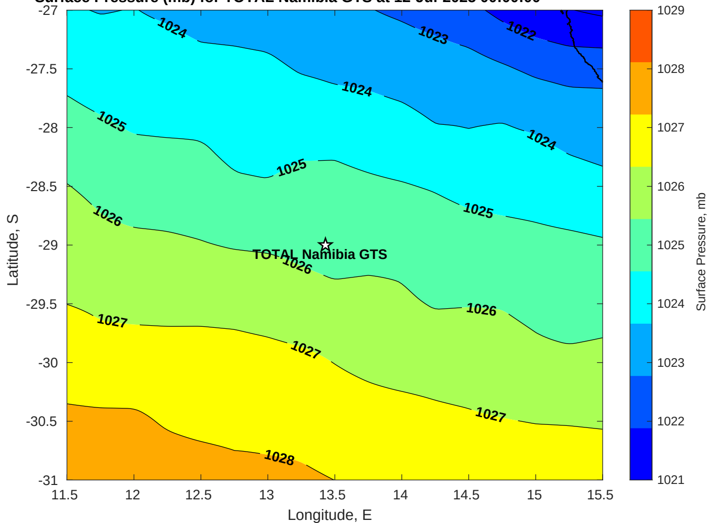
Surface Pressure (mb) for TOTAL Namibia GTS at 12-Jul-2025 00:00:00
