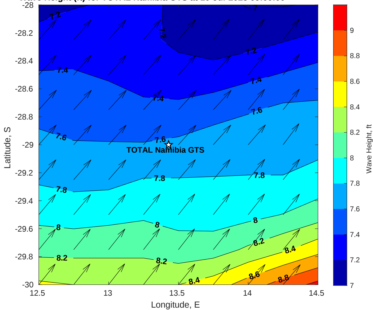
Wave Height (ft) for TOTAL Namibia GTS at 10-Jul-2025 09:00:00
