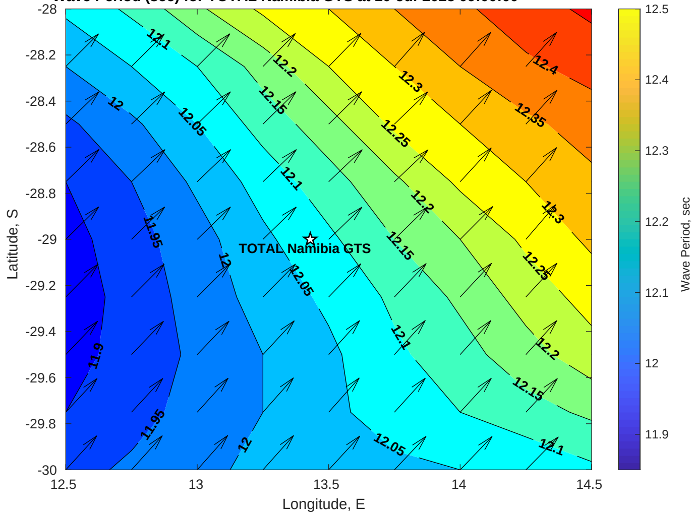
Wave Period (sec) for TOTAL Namibia GTS at 10-Jul-2025 09:00:00
