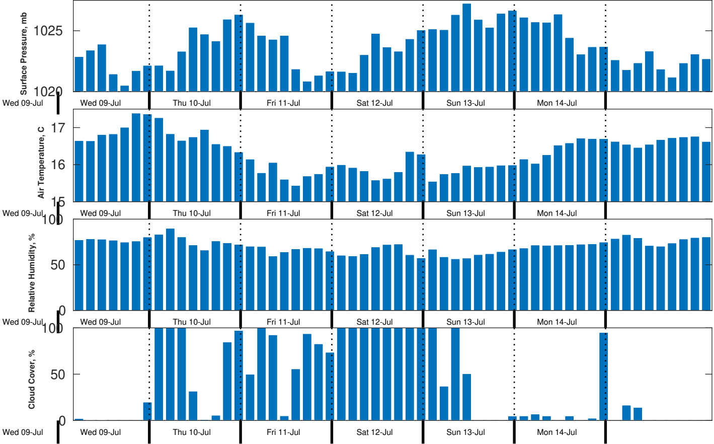
Met Forecast for TOTAL Namibia GTS from 10-Jul-2025 00:00:00 to 17-Jul-2025 00:00:00
