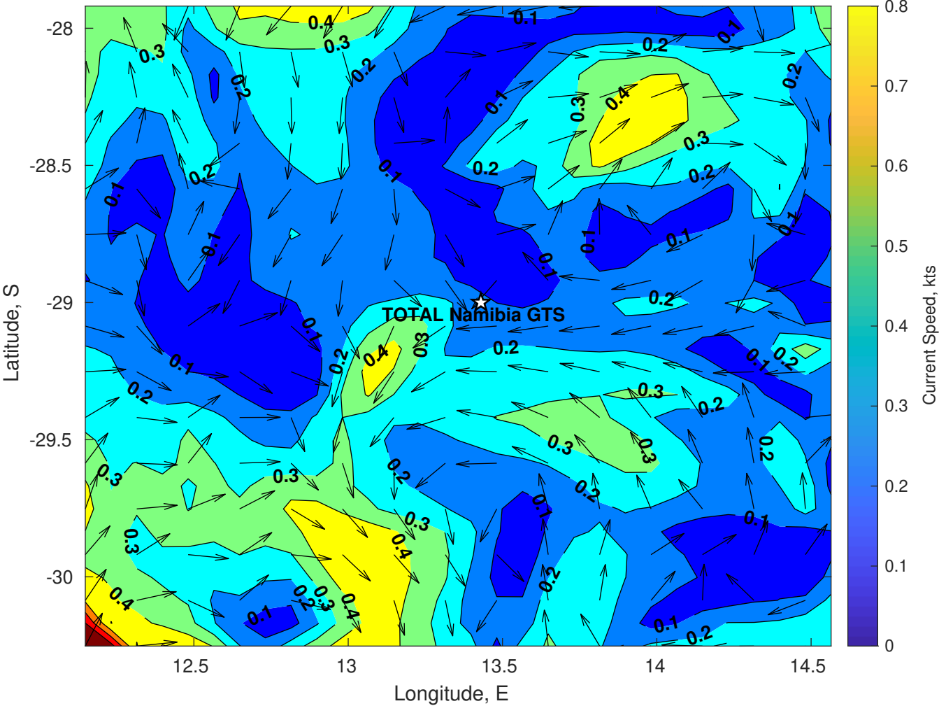
Surface Currents for TOTAL Namibia GTS at 09-Jul-2025 00:00:00
