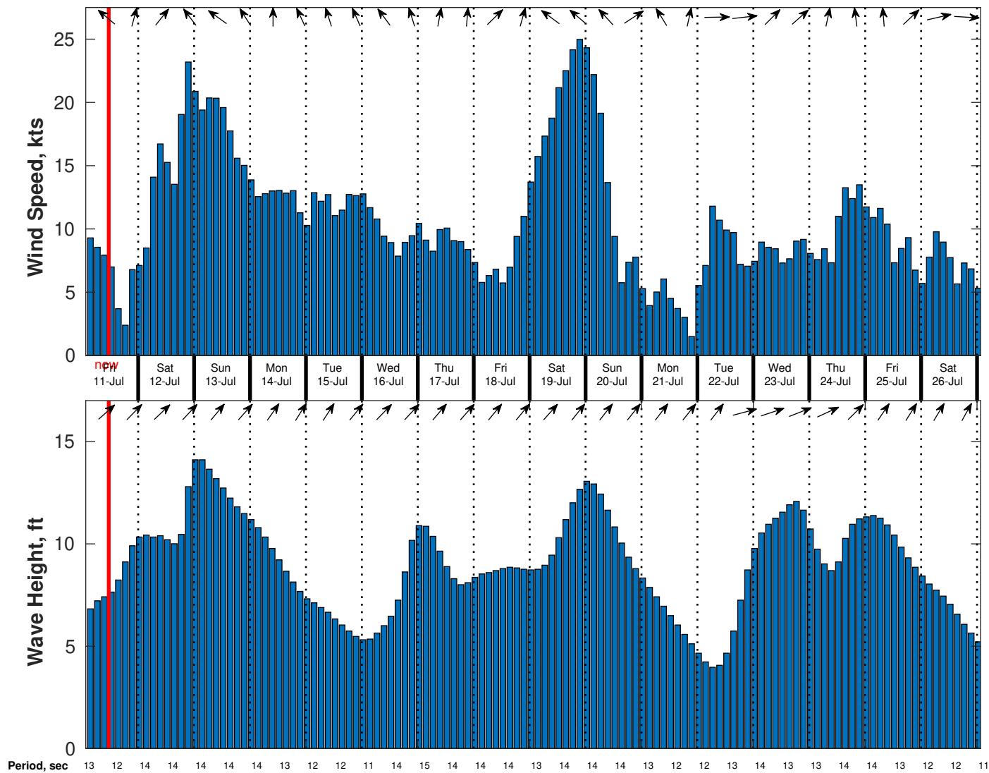
Wind & Wave Forecast for TOTAL Namibia GTS from 10-Jul-2025 02:00:00 to 26-Jul-2025 02:00:00
