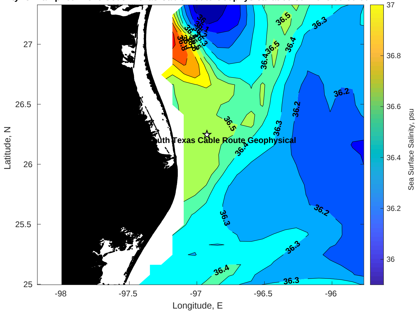
Surface Salinity for Tampnet P2378 South Texas Cable Route Geophysical at 09-Jul-2025 00:00:00
