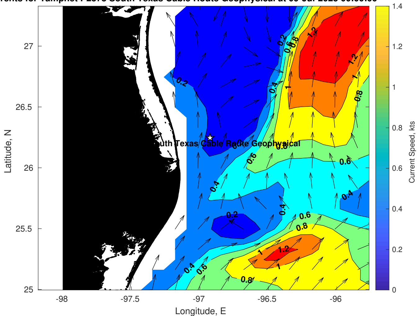
Surface Currents for Tampnet P2378 South Texas Cable Route Geophysical at 09-Jul-2025 00:00:00
