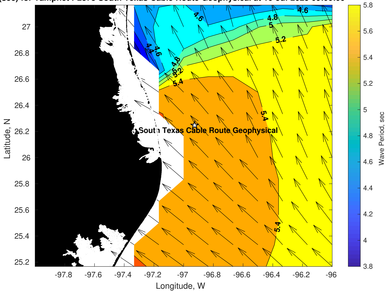
Wave Period (sec) for Tampnet P2378 South Texas Cable Route Geophysical at 10-Jul-2025 09:00:00
