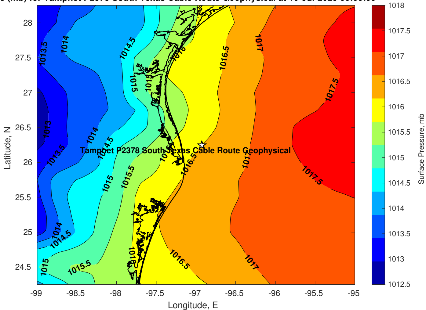
Pressure (mb) for Tampnet P2378 South Texas Cable Route Geophysical at 10-Jul-2025 00:00:00
