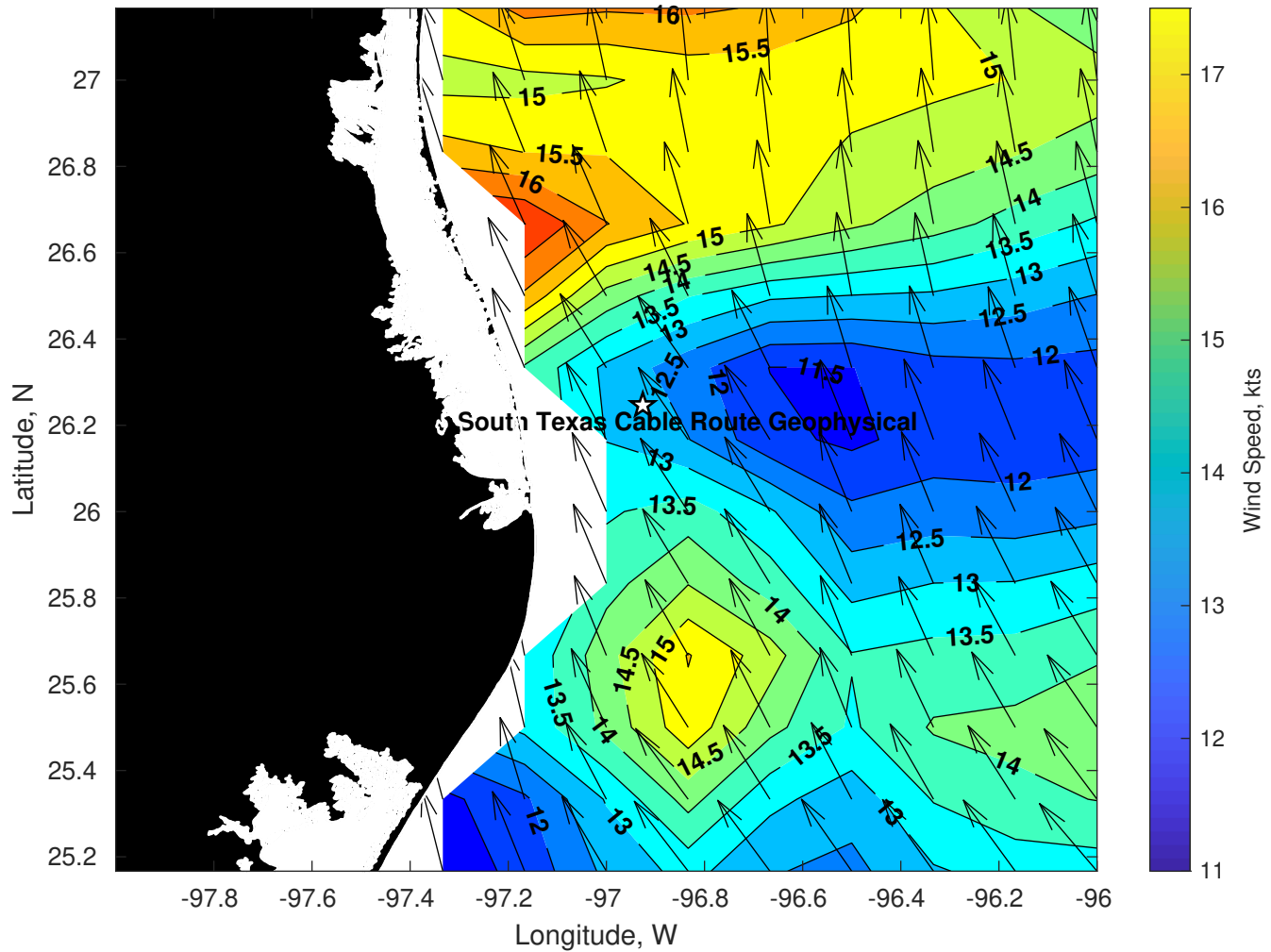
Winds (kts) for Tampnet P2378 South Texas Cable Route Geophysical at 10-Jul-2025 09:00:00
