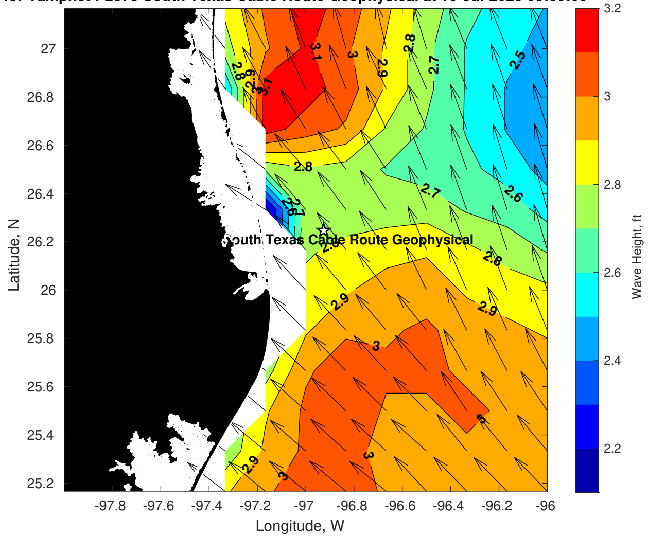
Wave Height (ft) for Tampnet P2378 South Texas Cable Route Geophysical at 10-Jul-2025 09:00:00
