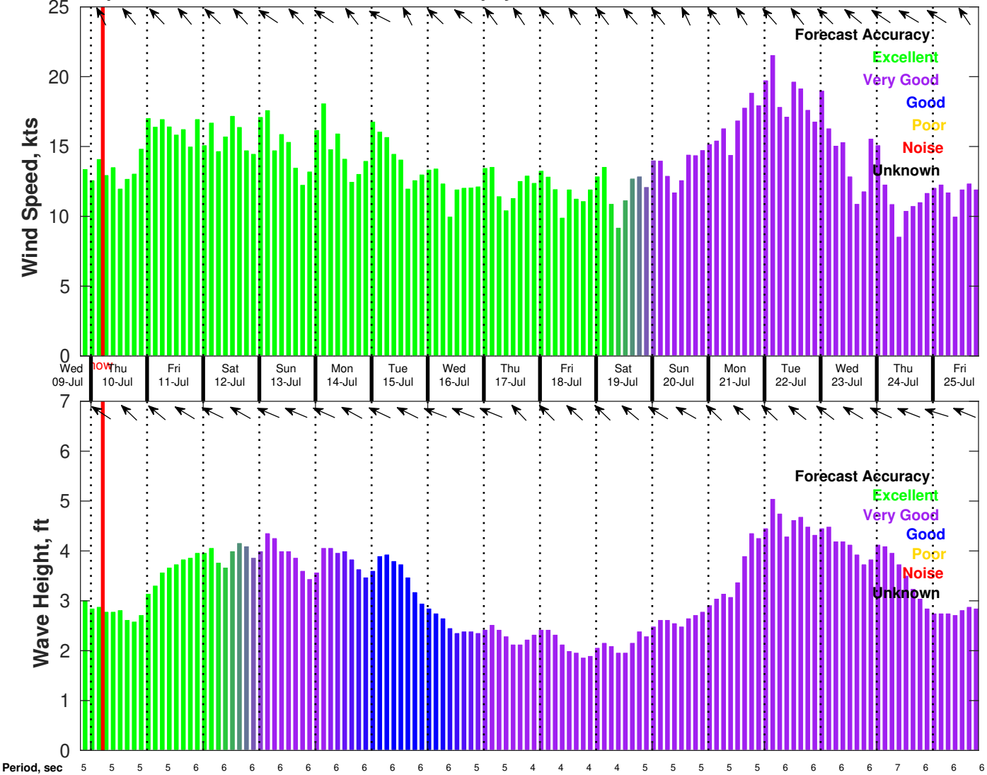
Wind & Wave Forecast for Tampnet P2378 South Texas Cable Route Geophysical from 09-Jul-2025 20:00:00 to 25-Jul-2025 20:00:00
