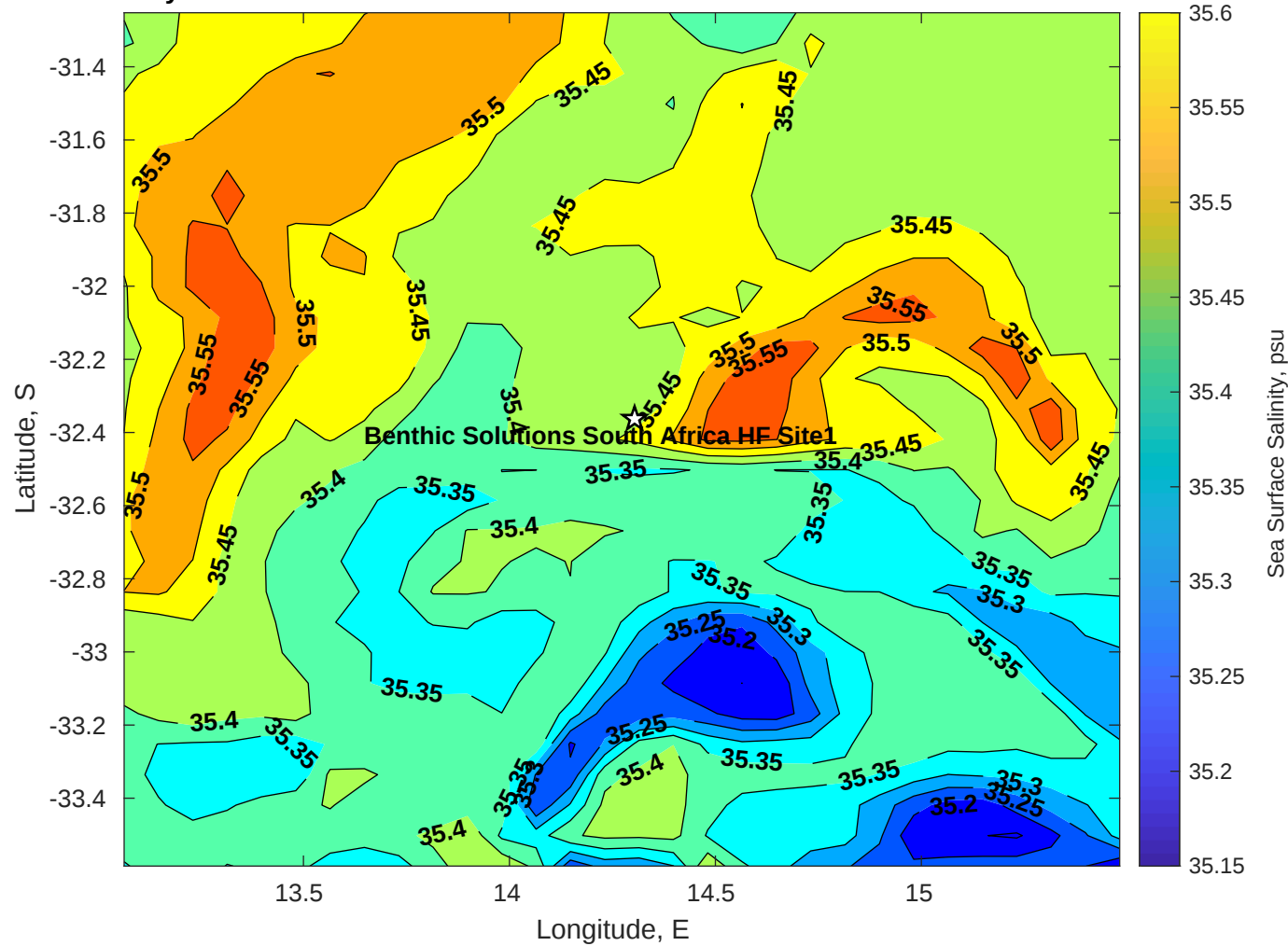
Surface Salinity for Benthic Solutions South Africa HF Site1 at 10-Jul-2025 00:00:00
