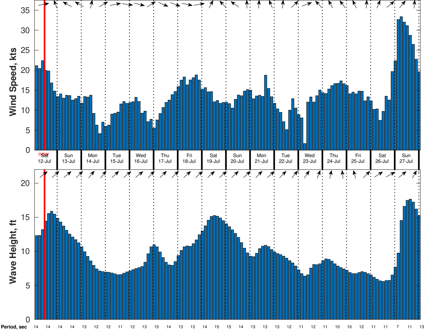
Wind & Wave Forecast for Benthic Solutions South Africa HF Site1 from 11-Jul-2025 02:00:00 to 27-Jul-2025 02:00:00
