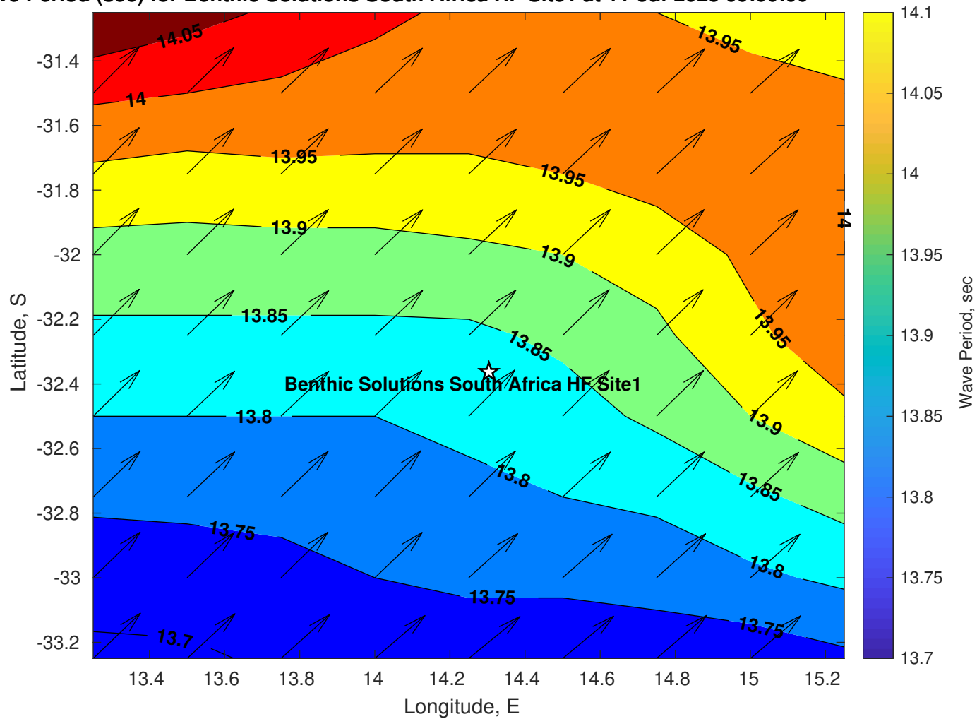
Wave Period (sec) for Benthic Solutions South Africa HF Site1 at 11-Jul-2025 09:00:00
