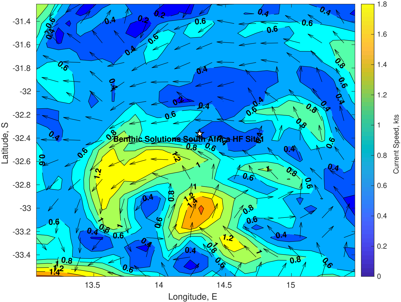
Surface Currents for Benthic Solutions South Africa HF Site1 at 10-Jul-2025 00:00:00
