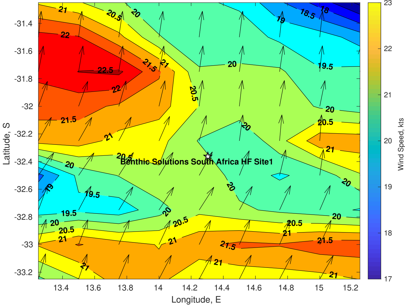
Winds (kts) for Benthic Solutions South Africa HF Site1 at 11-Jul-2025 09:00:00
