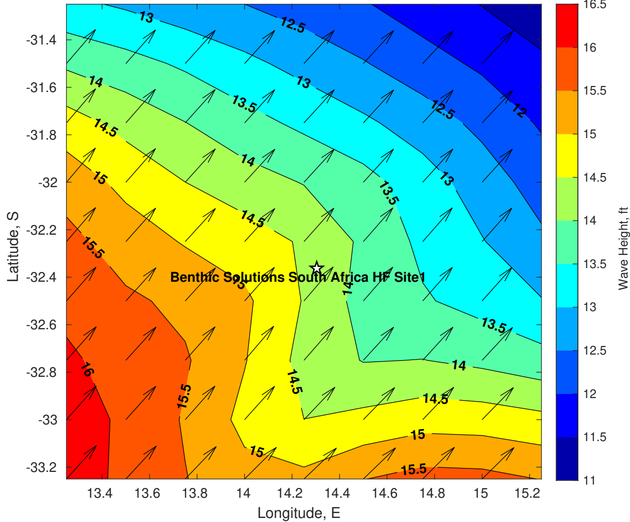
Wave Height (ft) for Benthic Solutions South Africa HF Site1 at 11-Jul-2025 09:00:00
