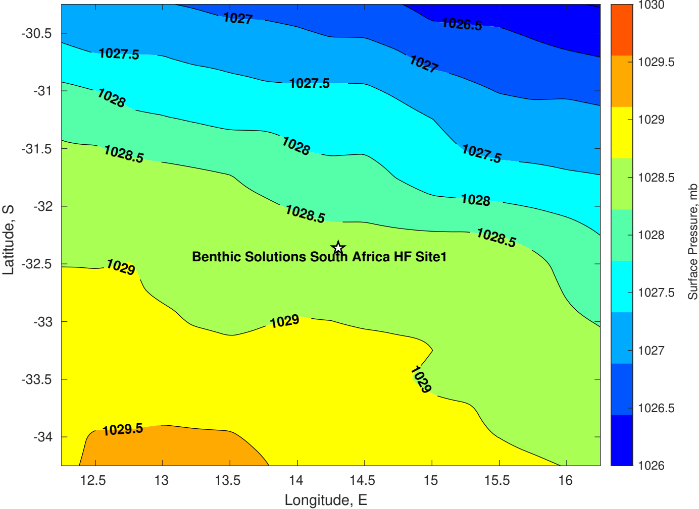
Surface Pressure (mb) for Benthic Solutions South Africa HF Site1 at 12-Jul-2025 00:00:00
