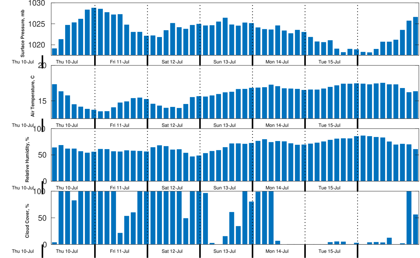
Met Forecast for Benthic Solutions South Africa HF Site1 from 11-Jul-2025 00:00:00 to 18-Jul-2025 00:00:00
