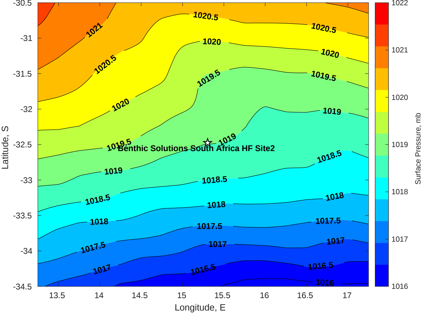
Surface Pressure (mb) for Benthic Solutions South Africa HF Site2 at 11-Jul-2025 00:00:00
