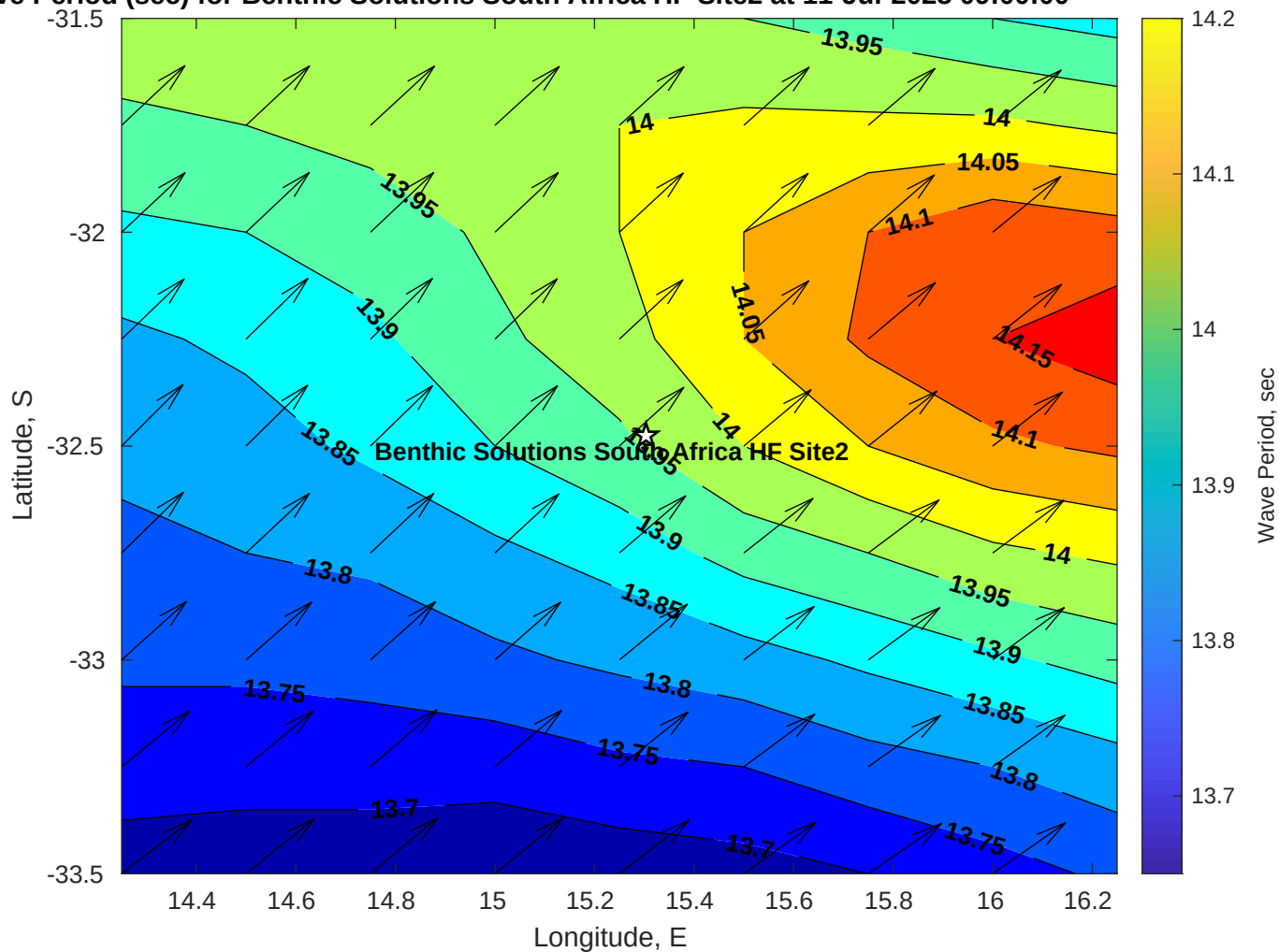
Wave Period (sec) for Benthic Solutions South Africa HF Site2 at 11-Jul-2025 09:00:00
