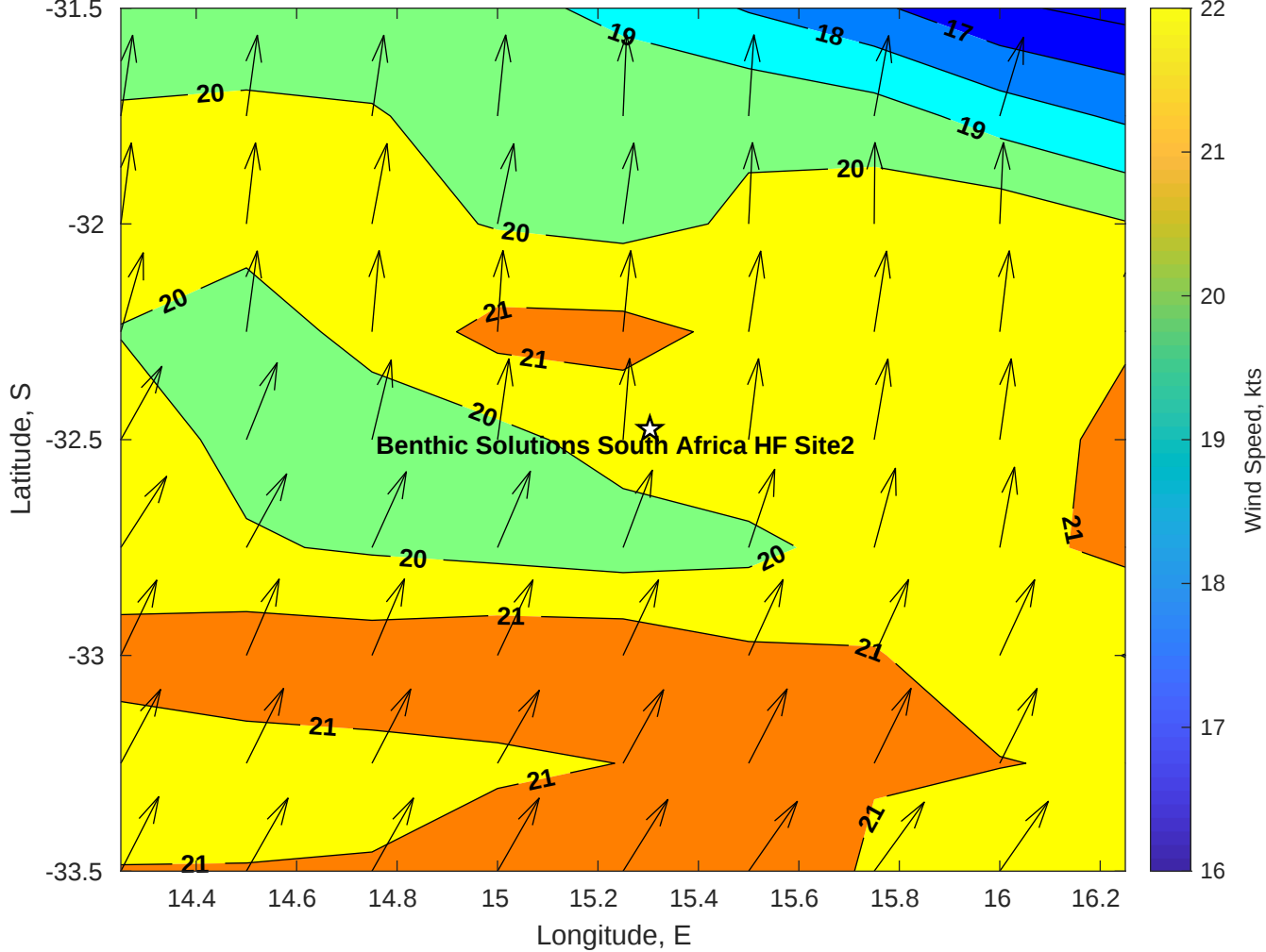
Winds (kts) for Benthic Solutions South Africa HF Site2 at 11-Jul-2025 09:00:00
