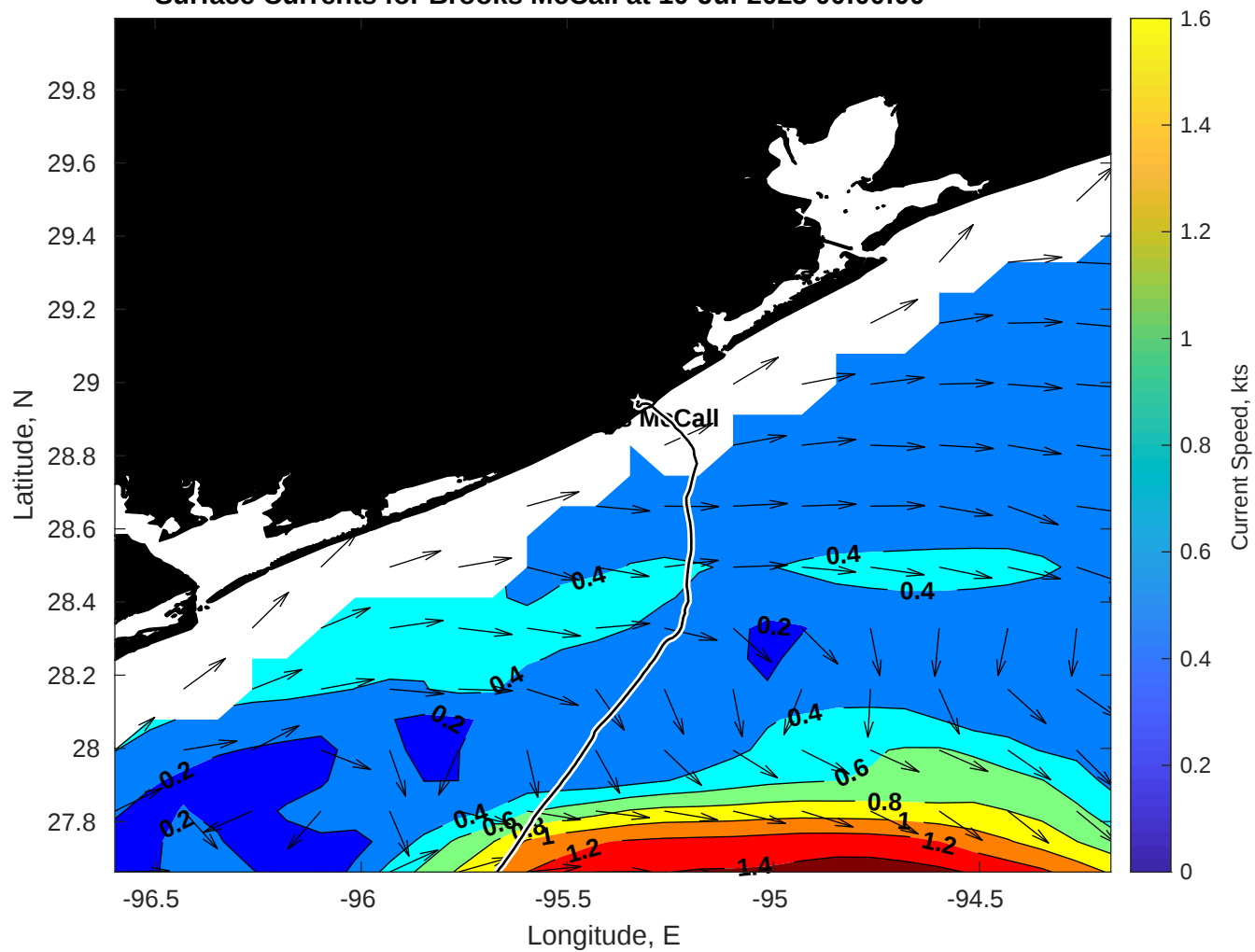
Surface Currents for Brooks McCall at 10-Jul-2025 00:00:00
