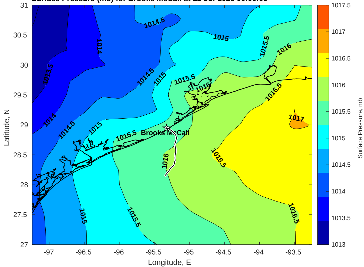
Surface Pressure (mb) for Brooks McCall at 11-Jul-2025 00:00:00
