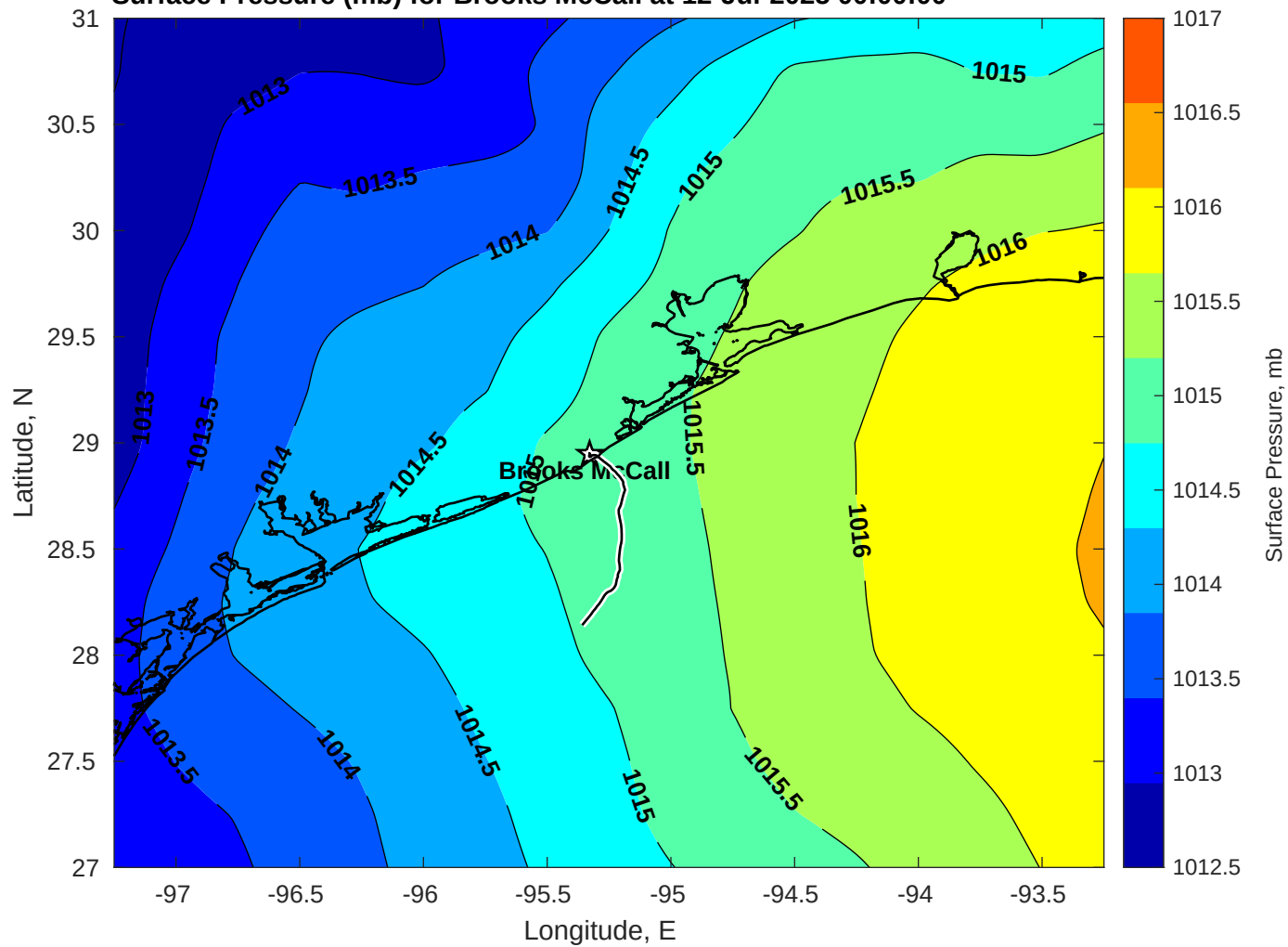
Surface Pressure (mb) for Brooks McCall at 12-Jul-2025 00:00:00
