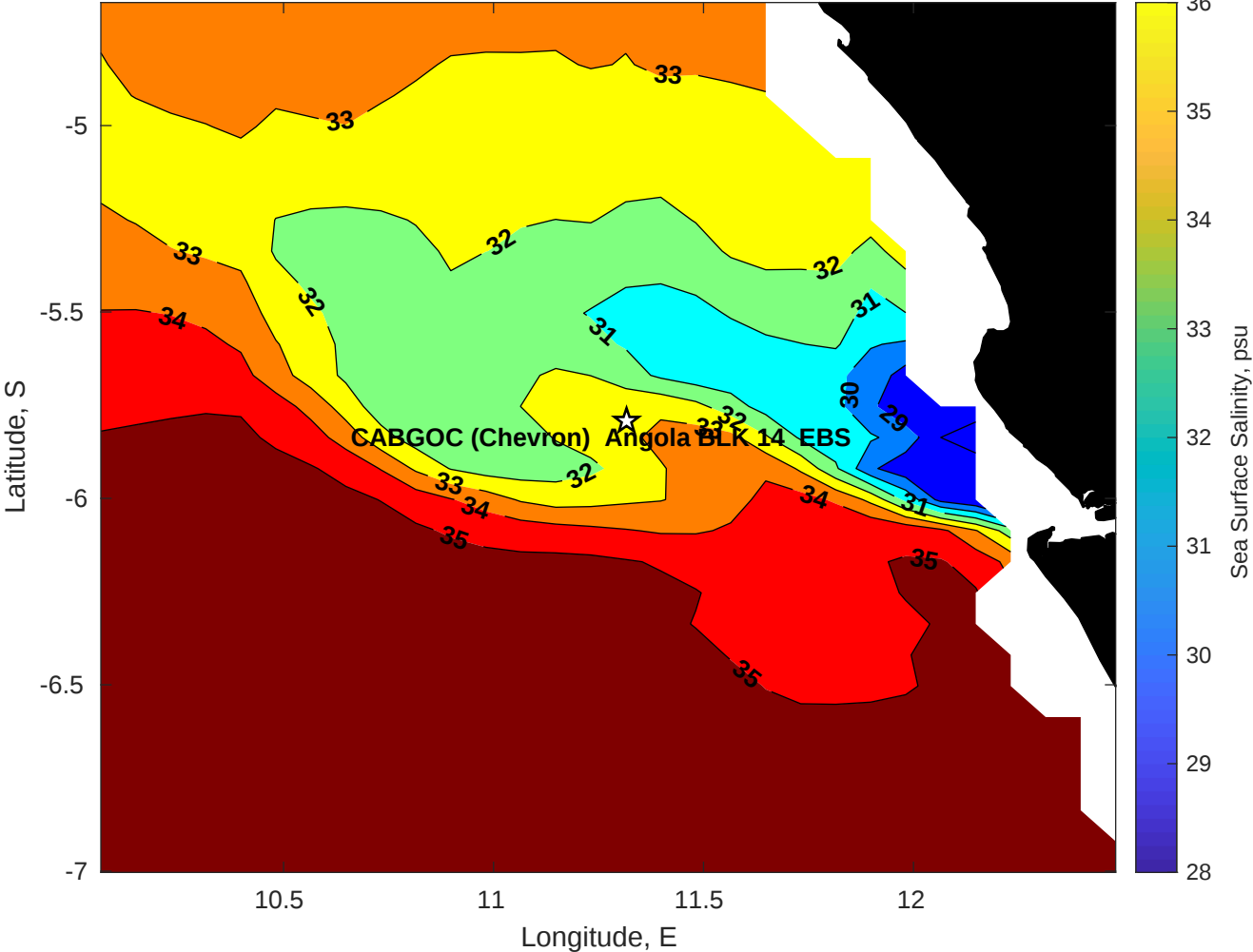
Surface Salinity for CABGOC (Chevron) Angola BLK 14 EBS at 10-Jul-2025 00:00:00
