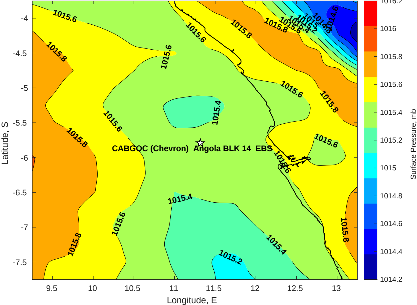
Surface Pressure (mb) for CABGOC (Chevron) Angola BLK 14 EBS at 12-Jul-2025 00:00:00
