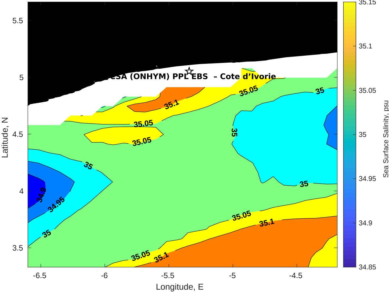
Surface Salinity for CSA (ONHYM) PPL EBS - Cote d'Ivoire at 10-Jul-2025 00:00:00
