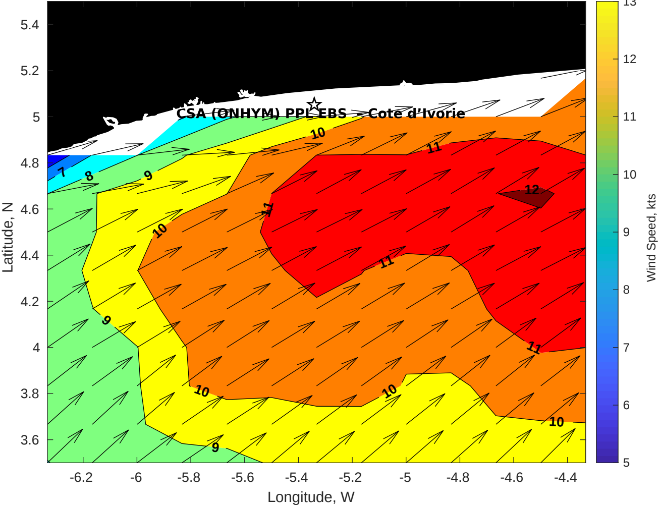
Winds (kts) for CSA (ONHYM) PPL EBS - Cote d'Ivoire at 11-Jul-2025 09:00:00
